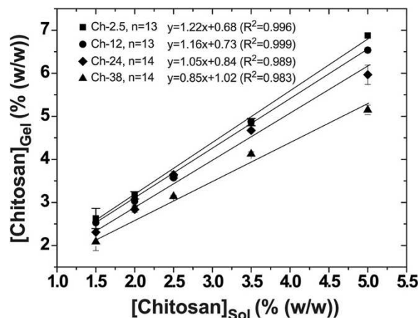
Figure 1. Final hydrogel concentration ( [\text{Chitosan}]_{\text{Gel}} ) after neutralization with a NaOH solution (3 M, 1 h) and autoclave sterilization, with different degrees of acetylation (Ch-2.5, Ch-12, Ch-24 and Ch-38 hydrogels) with different polymer solution concentrations ( [\text{Chitosan}]_{\text{Sol}} ).
