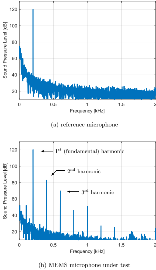
Figure 3: Spectra of the measured sound pressure (a) with the reference microphone, (b) with the MEMS microphone under test. Note that thanks to the harmonic control, there are no higher harmonics measured by the reference microphone.
