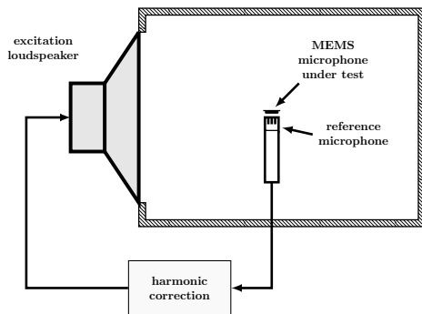
Figure 1: Simplified schema of the measurement setup.
