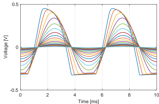
Figure 5: Time-domain signal of the voltage at the output of the MEMS microphone under test for different levels from 90 dB SPL to 128 dB SPL. Note that the electrical signals for the four highest sound pressure levels (122, 124, 126, and 128 dB SPL) are saturated.
