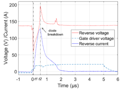
Fig. 7. Measurements during diode reverse breakdown.
