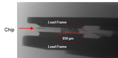
Fig. 5. One short-circuited diode of UD4KB80 bridge.
