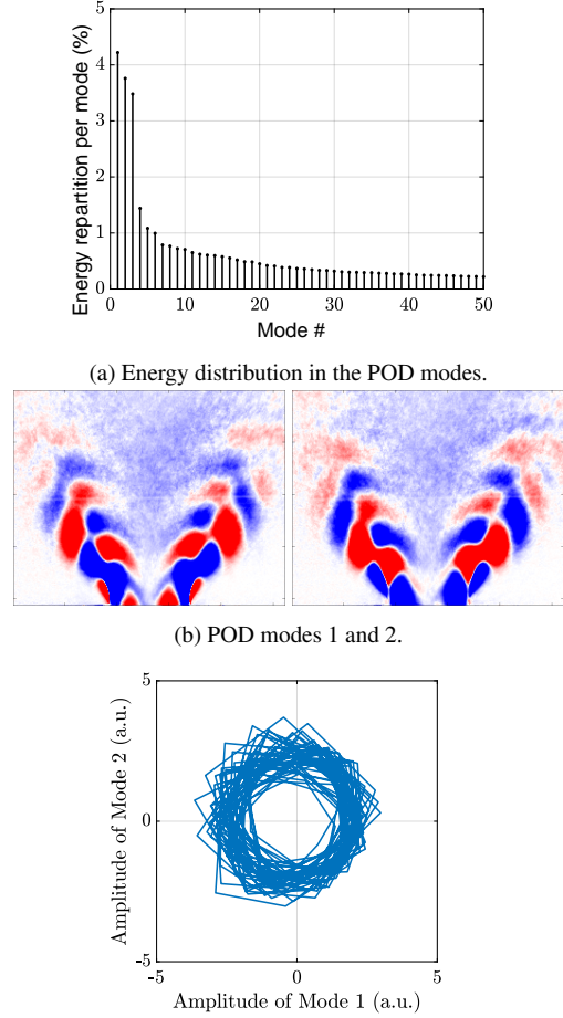
(a) Energy distribution in the POD modes. (b) POD modes 1 and 2. (c) a_2^v(t) , amplitude of POD mode 2, plotted against a_1^v(t) , amplitude of POD mode 1.
