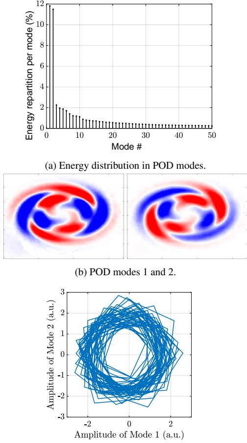
(a) Energy distribution in POD modes. (b) POD modes 1 and 2. (c) a_2^h(t) , amplitude of POD mode 2, plotted against a_1^h(t) , amplitude of POD mode 1.
