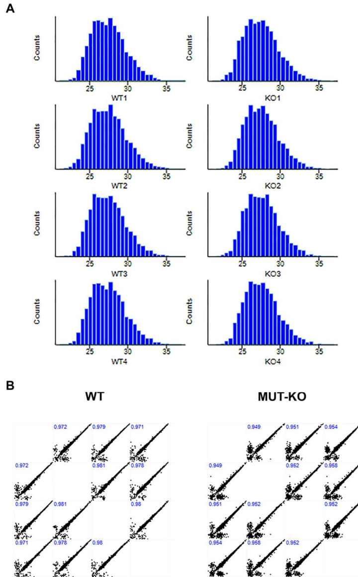
Fig. 2. The quality of the proteomic dataset acquired by LC-MS/MS analysis was checked in each replicate analysing (A) the normal distributions of LFQ intensities and (B) the correlation coefficients using Pearson's correlation.
