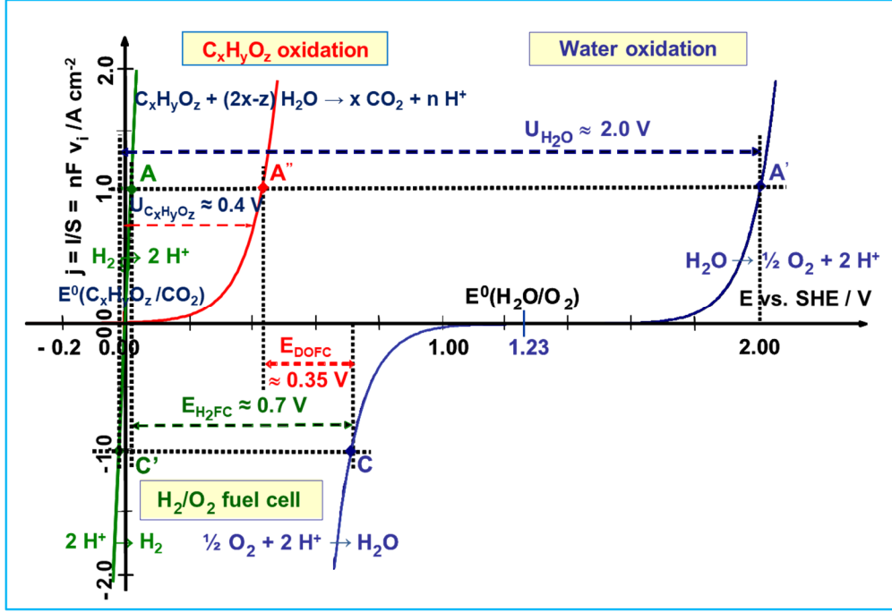
Fig.2: Theoretical electrical characteristics j(E) for a reaction kinetics controlled by the Butler-Volmer law ( \alpha = 0.5 , n = 2 ): \text{C}_x\text{H}_y\text{O}_z oxidation, \text{H}_2\text{O} oxidation, \text{O}_2 reduction and proton reduction. U_{\text{C}_x\text{H}_y\text{O}_z} , U_{\text{H}_2\text{O}} , E_{\text{DOFC}} and E_{\text{H}_2\text{FC}} are the cell voltages for \text{C}_x\text{H}_y\text{O}_z electrolysis, water electrolysis, direct oxidation fuel cell and hydrogen/oxygen fuel cell at a given current density j , e.g. 1 \text{ A cm}^{-2} .
