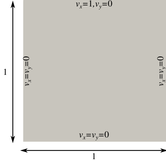
Figure 10: Boundary conditions for the 2D lid-driven cavity problem. Lengths are in millimeters and velocities in millimeters per millisecond.
