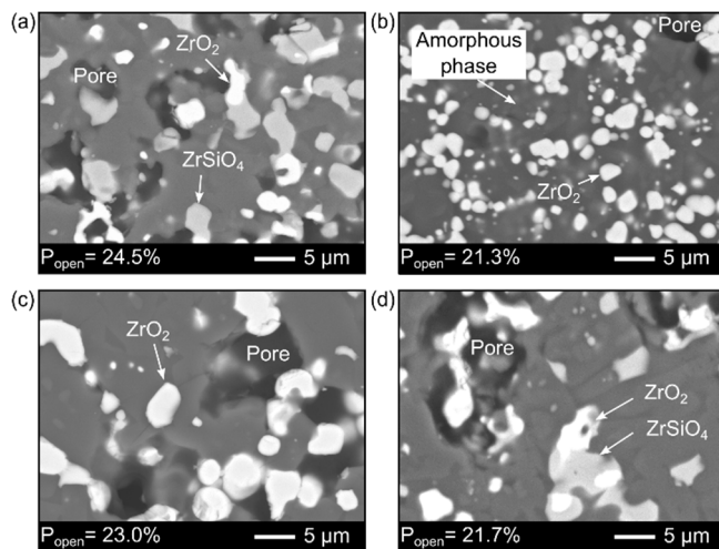
8 9 Fig. 4. SEM images showing the impact of additives (1 mol%) on the final microstructure and open porosity 10 ( P_{open} ) of zircon–alumina–andalusite mixtures sintered at 1550 °C: (a) without additives, (b) 0.34 wt% Na 2 O, (c) 11 0.88 wt% TiO 2 , and (d) 1.55 wt% P 2 O 5 .
