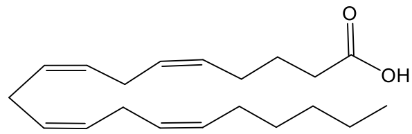
Arachidonic acid (20:4n-6)
