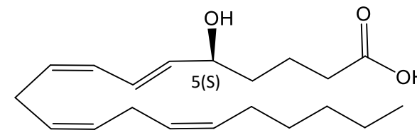
5(S)-OH-6E,8Z,11Z,14Z-20:4 (5-HETE)
