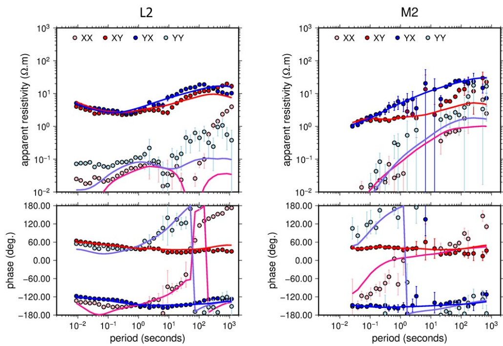
Figure 2: MT soundings for sites L2 (left panel) and M2 (right panel). The upper and lower panels display the apparent resistivity in \Omega.m and phase in degrees, respectively. The full lines signify the responses of the best-fitting model.
