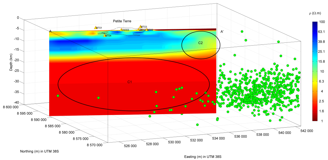
Figure 4: N120° cross-section through the 3D resistivity volume obtained from the inversion of the land and marine MT data. Green circles represent the hypocenters of the seismic events recorded from May 1, 2018, to May 28, 2019 (Lemoine et al., 2019). Yellow triangles represent the MT sites used in the MT inversion.
