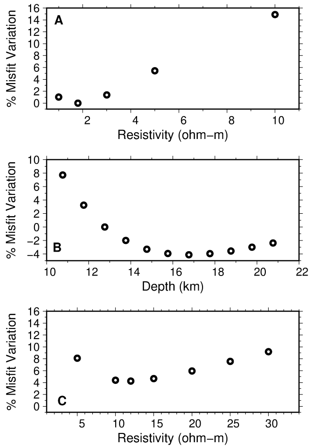
Figure 5: Variation of the misfit between the tested and preferred model as a function of a) the resistivity of the deep conductive layer, b) the depth of the top of this conductor and c) the presence of a conductor between 5 and 13km depth to the South-East of Petite Terre. The value 0 corresponds to the preferred model.
