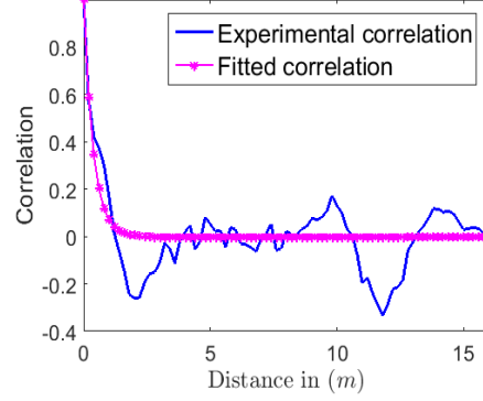
Figure 17: Experimental and fitted correlation of W(\%)
