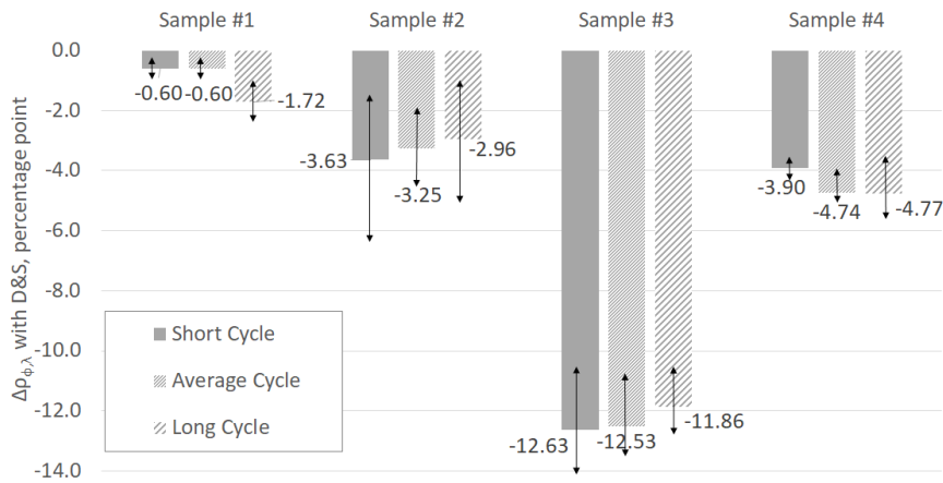
FIGURE 2.A. Specular reflectance ( \Delta\rho_{\lambda,\phi} ) losses for samples #1 to #4 in function of their cycle duration
