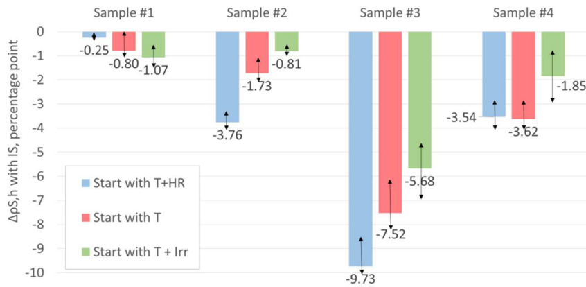
FIGURE 3.B. Solar-weighted hemispherical reflectance ( \Delta\rho_{s,h} ) losses for samples #1 to #4 in function of the initial stress encountered
