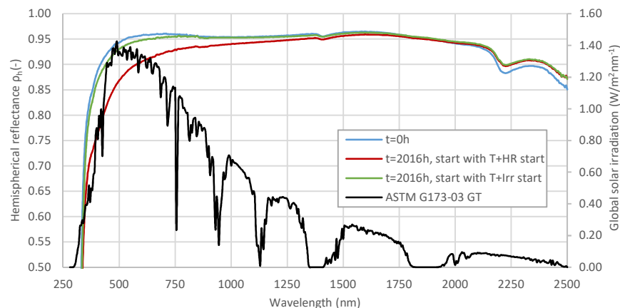
FIGURE 5. Spectral hemispherical reflectance \rho_{\lambda,h} of sample #3 at t=0 and t=2016 for long cycle and two different initialization.
