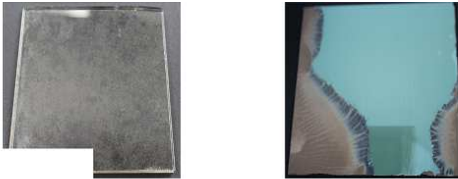
FIGURE 4 : Left : Reflective face of sample #4 at t=2016h (short rotation, start with T). Right : paint side on sample #1, after the same conditions than previously.
