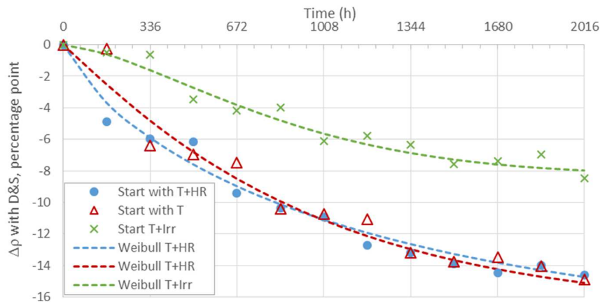
FIGURE 6. Weibull distribution of \rho_{\lambda,\varphi} for manufacturer #3 mirrors, aging with 12 short cycles (168h)
