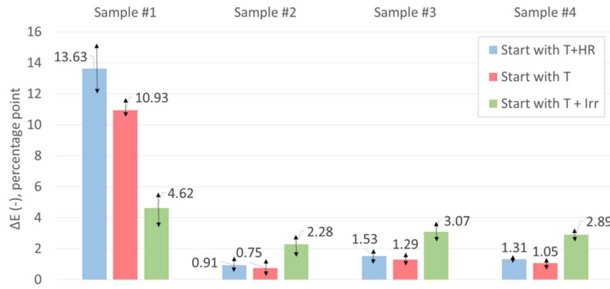
FIGURE 3.C. Colorimetric degradation ( \Delta E ) losses for samples #1 to #4 in function of the initial stress encountered
