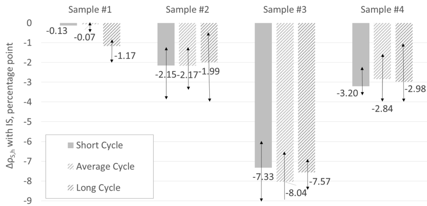
FIGURE 2.B. Solar-weighted hemispherical reflectance ( \Delta\rho_{s,h} ) losses for samples #1 to #4 in function of their cycle duration
