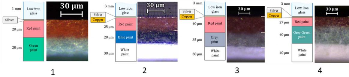
FIGURE 1. Samples presentation from manufacturers #1, #2, #3 and #4 [39].
