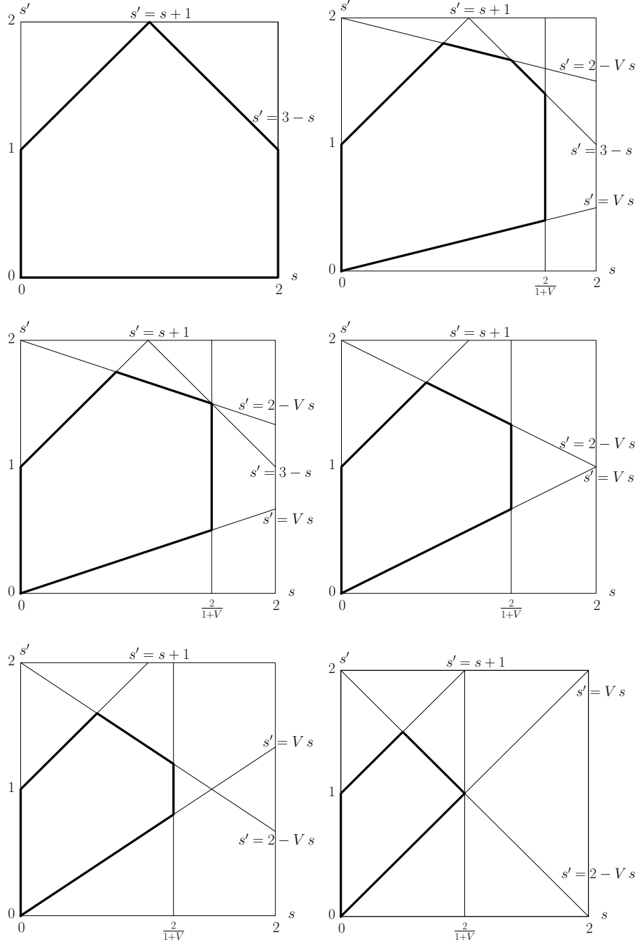
Figure 2: Necessary stability regions described by the inequalities (17) for V = 0 , V = \frac{1}{4} [first line, from left to right], V = \frac{1}{3} , V = \frac{1}{2} [second line, from left to right], and for V = \frac{2}{3} , V = 1 [third line, from left to right].
