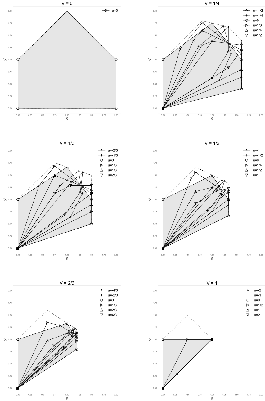
Figure 3: Numerical study of necessary and sufficient stability regions
