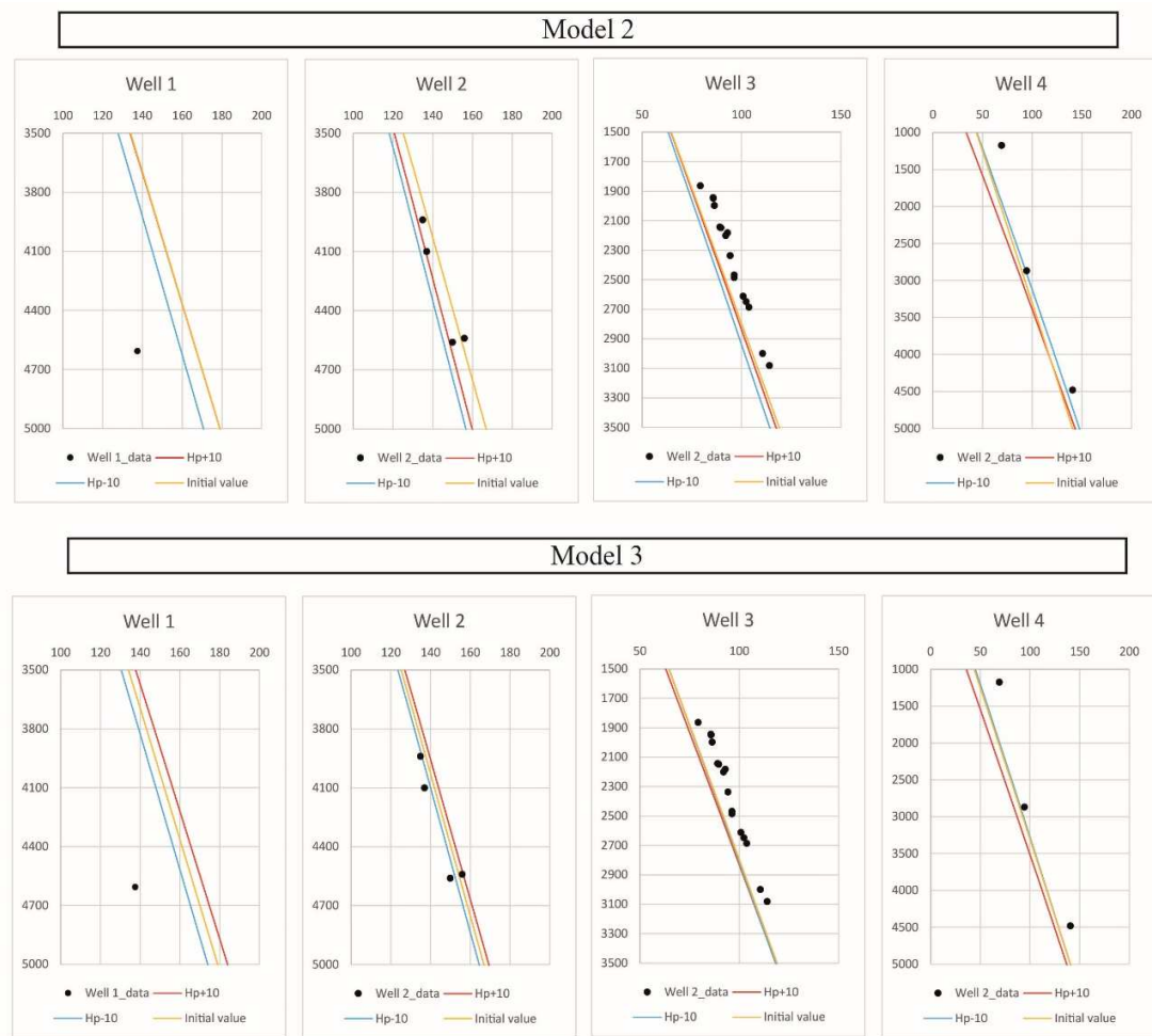
Appendix D2: We tested the sensitivity of varied radiogenic heat production on model 2 and 3. We performed a 10% variation test for all the layers together. In orange are the reference radiogenic heat production as stated in table 1. In red and blue are the sensitivity test of +10% and -10% radiogenic heat production, respectively.
