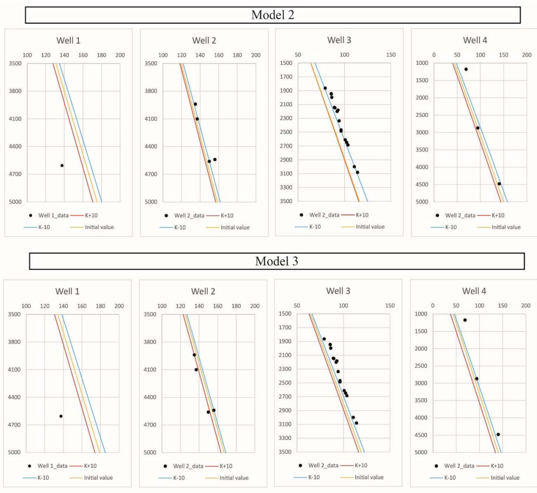
Appendix C2: We tested the sensitivity of varied thermal conductivity on model 2 and 3. We performed a 10% variation test for all the layers. In orange are the reference thermal conductivity as stated in table 1. In red and blue are the sensitivity test of +10% and -10% thermal conductivity, respectively.
