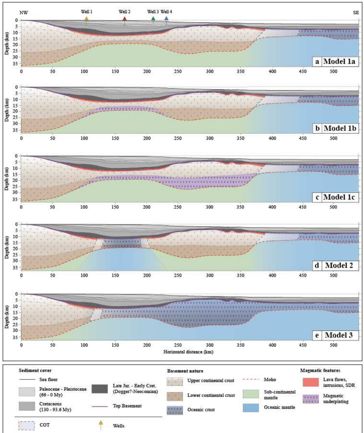
Figure 5: Schematic representations of the five tested models. The origin of the crust in the Zambezi Depression may be a ) entirely continental without magmatic underplating (Model 1a), b ) continental with
