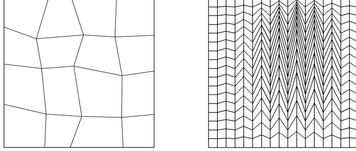
Figure 2: First deformed quadrilateral mesh on left and first Kershaw mesh on right.
