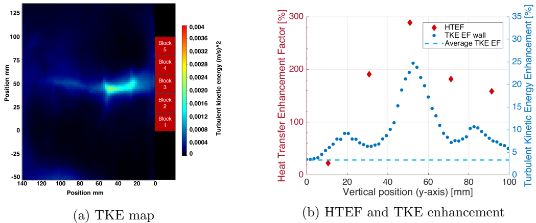
Figure 12: Results for configuration n°3b ( f = 25 kHz, perpendicular to the water flow, P_{US} = 52.5 W + f = 2 MHz, collinear, P_{US} = 52.5 W)
