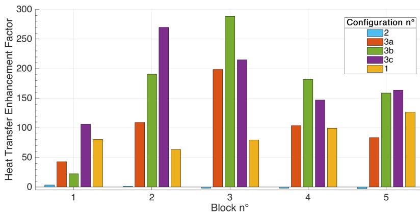
Figure 14: Heat Transfer Enhancement Factor for each power distribution per emitter, total power is constant P_{US} = 105 W
