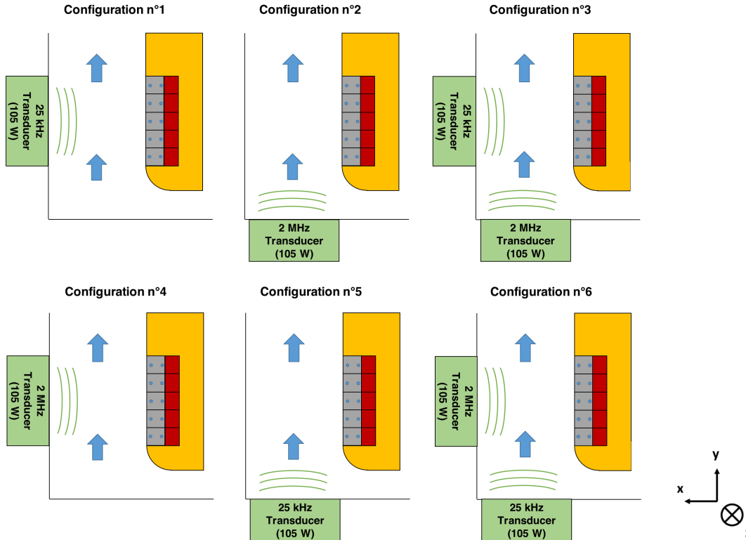
Figure 2: Scheme of the six experimental configurations
