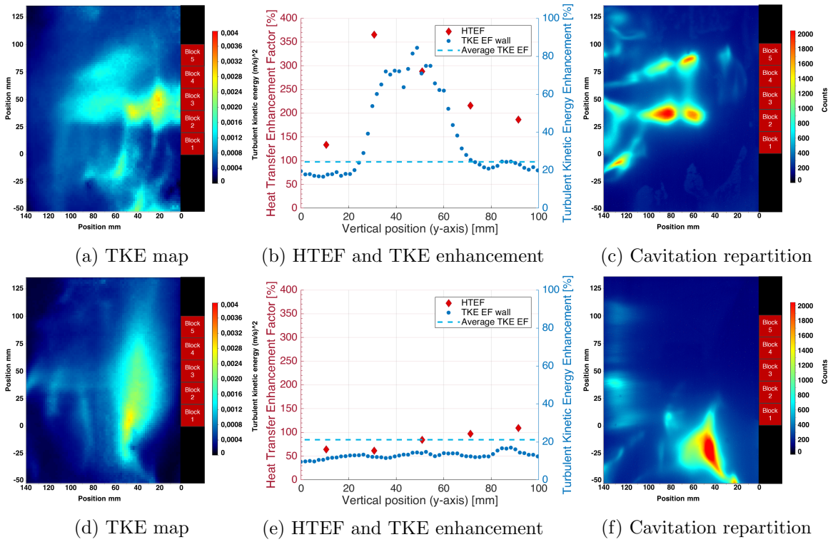
Figure 9: (a), (b), (c) : Results for configuration n°3 ( f = 25 kHz, perpendicular to the water flow, P_{US}=105 W + f = 2 MHz, collinear, P_{US}=105 W) // (d), (e), (f) : Results for configuration n°6 ( f = 2 MHz, perpendicular to the water flow, P_{US}=105 W + f = 25 kHz, collinear, P_{US}=105 W)
