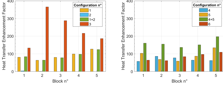
Figure 10: Heat Transfer Enhancement Factor for each configuration
