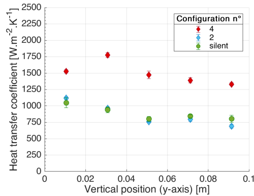
Figure 6: Influence of high-frequency ultrasound on heat transfer coefficients along heating wall ( f = 2 MHz, P_{US} = 105 W)
