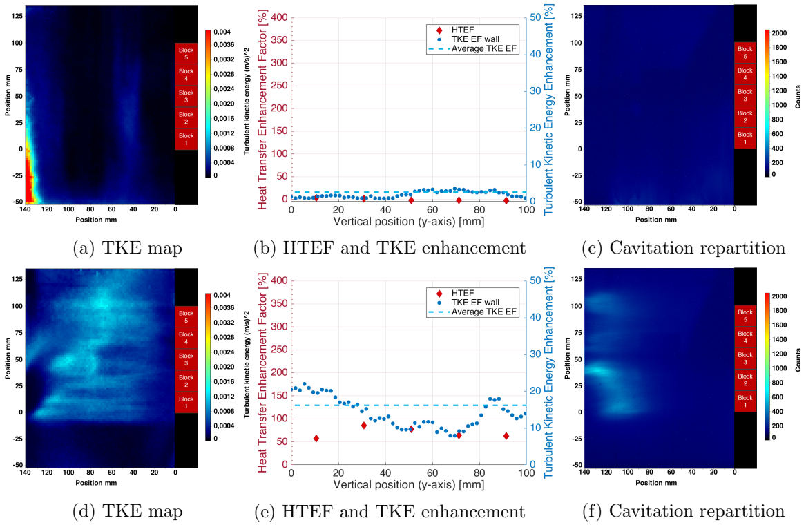
Figure 7: (a), (b), (c) : Results for configuration n°2 ( f = 2 MHz, collinear to the water flow, P_{US} = 105 W) // (d), (e), (f) : Results for configuration n°4 ( f = 2 MHz, perpendicular to the water flow, P_{US} = 105 W)
