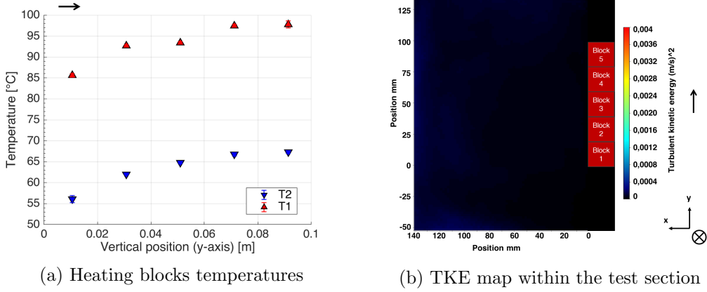
Figure 3: Temperature profile (a) and Turbulent Kinetic Energy (b) in silent conditions
