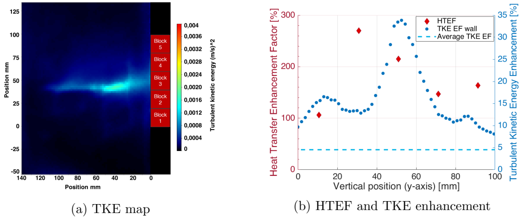
Figure 13: Results for configuration n°3b ( f = 25 kHz, perpendicular to the water flow, P_{US} = 73.5 W + f = 2 MHz, collinear, P_{US}=31.5 W)
