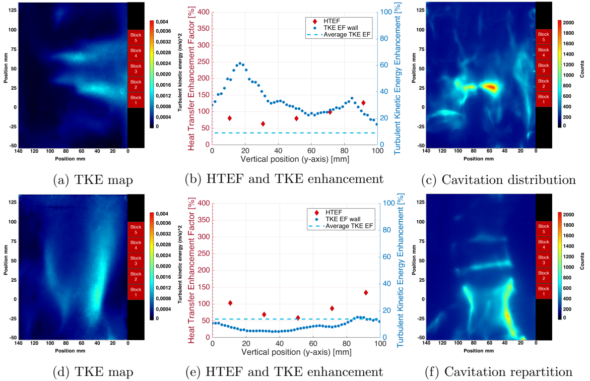
Figure 5: (a), (b), (c) : Results for configuration n°1 ( f = 25 kHz, perpendicular to the water flow, P_{US} = 105 W) // (d), (e), (f) : Results for configuration n°5 ( f = 25 kHz, collinear to the water flow, P_{US} = 105 W)
