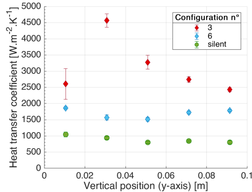
Figure 8: Influence of dual low-high frequency ultrasound on heat transfer coefficient ( f=25 kHz, P_{US}=105 W + f=2 MHz, P_{US}=105 W)
