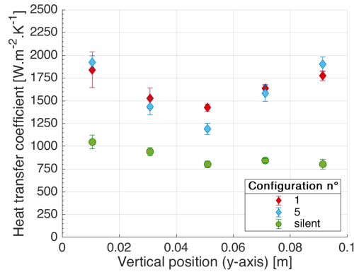
Figure 4: Influence of low-frequency ultrasound on heat transfer coefficients along heating wall ( f = 25 \text{ kHz} , P_{\text{US}} = 105 \text{ W} )
