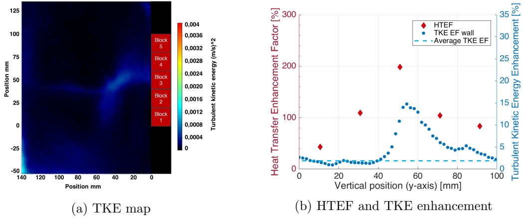
Figure 11: Results for configuration n°3a ( f = 25 kHz, perpendicular to the water flow, P_{US} = 31.5 W + f = 2 MHz, collinear, P_{US} = 73.5 W)
