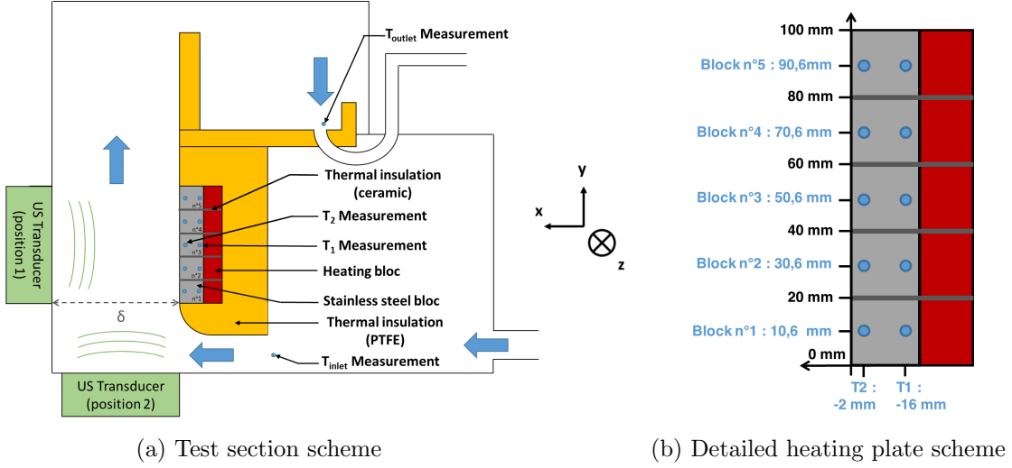
Figure 1: Test section design
