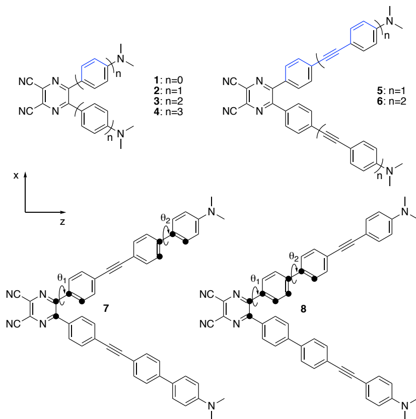
Figure 1: Pyrazine derivatives investigated in this work. The Cartesian frame used in NLO calculations is shown on the left. The dihedral angles around single bonds ( \theta_{1-3} ) are defined between dotted carbon atoms starting from the pyrazine core, as exemplified on compounds 7 and 8 . The conjugated segment considered to compute the BLA is shown in blue in compounds 1-6 .
