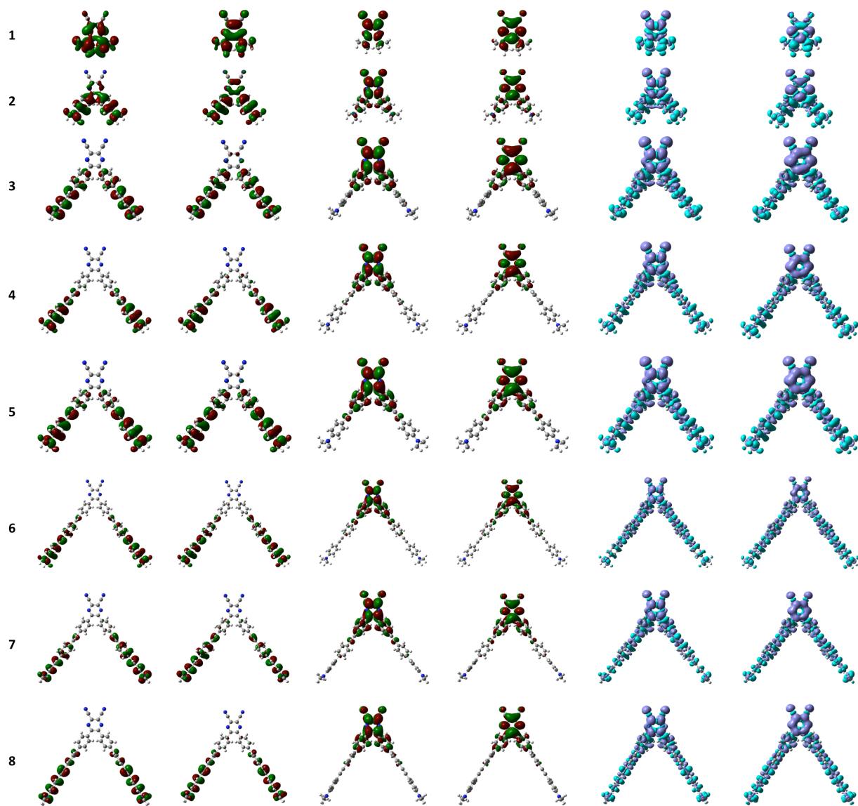
Figure 3: From left to right: HOMO-1, HOMO, LUMO and LUMO+1 of the eight pyrazine derivatives, and electron density differences associated to the S_0 \rightarrow S_1 and S_0 \rightarrow S_2 transitions. Dark (light) blue lobes in density maps are associated with positive (negative) \Delta\rho values.
