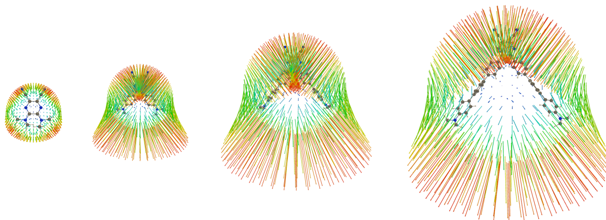
Figure 5: Unit-sphere representation of the static first hyperpolarizability calculated at the TDDFT/M06-2X/6-311+G(d) for compounds 1 to 4 (from left to right). Arrows represent the magnitude of the second-order contribution to the induced dipole when an external field is applied normally to the surface of a virtual sphere centered on the center of mass of the molecules. See SI and Figure S10 for details on the USR and color scales.
