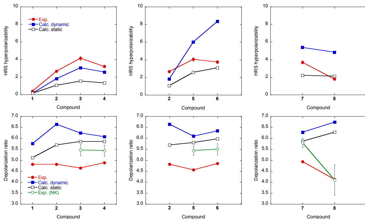
Figure 4: Evolution of the HRS hyperpolarizability (in 10^4 a.u., top) and depolarization ratio (bottom) in the series of compounds 1-4 (left), 2,5,6 (middle) and 7-8 (right).
