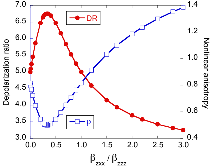
Figure 2: Evolution of the depolarization and anisotropy ratios as a function of R = \beta_{zxx}/\beta_{zzz} when assuming both C_{2v} and Kleinman symmetries (equations 9 and 14).
