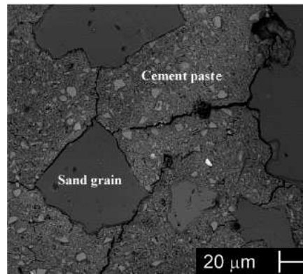
Figure 10. Cracking at the mortar scale [60].
