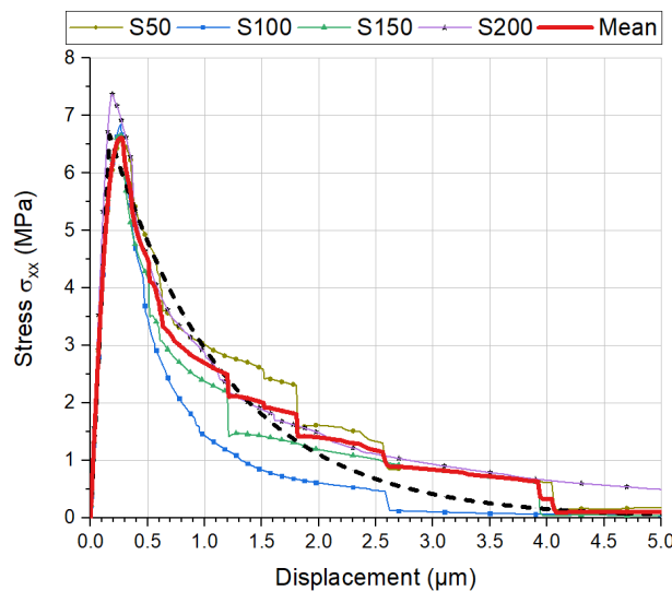
308 309 310 Figure 9. The stress-crack opening displacement curve of the cement paste microstructure 311 (CEM I, w/c = 0.45) using intrinsic micromechanical parameters (dashed line = idealised 312 behaviour of a finite element representing cement paste at the scale of mortar).
