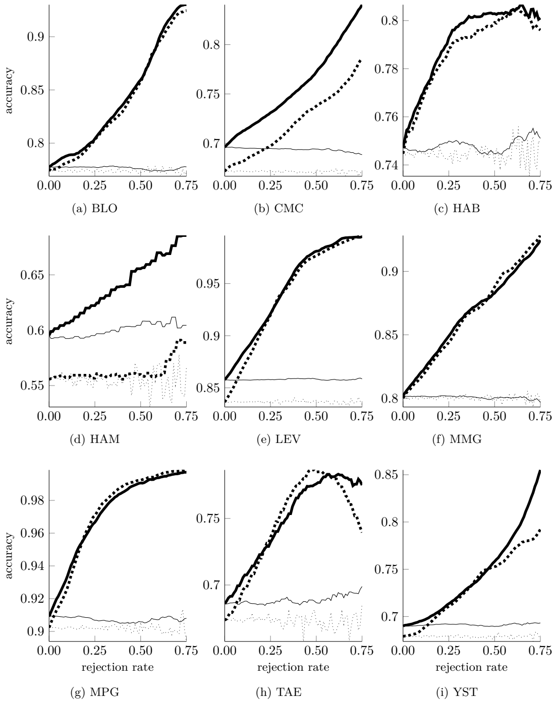
Figure 7: Accuracy-rejection curves based on the ignorance of ECR (—) and of ELR (— · —), and based on randomly rejecting test instances classified by ECR (—) and by ELR (···).
