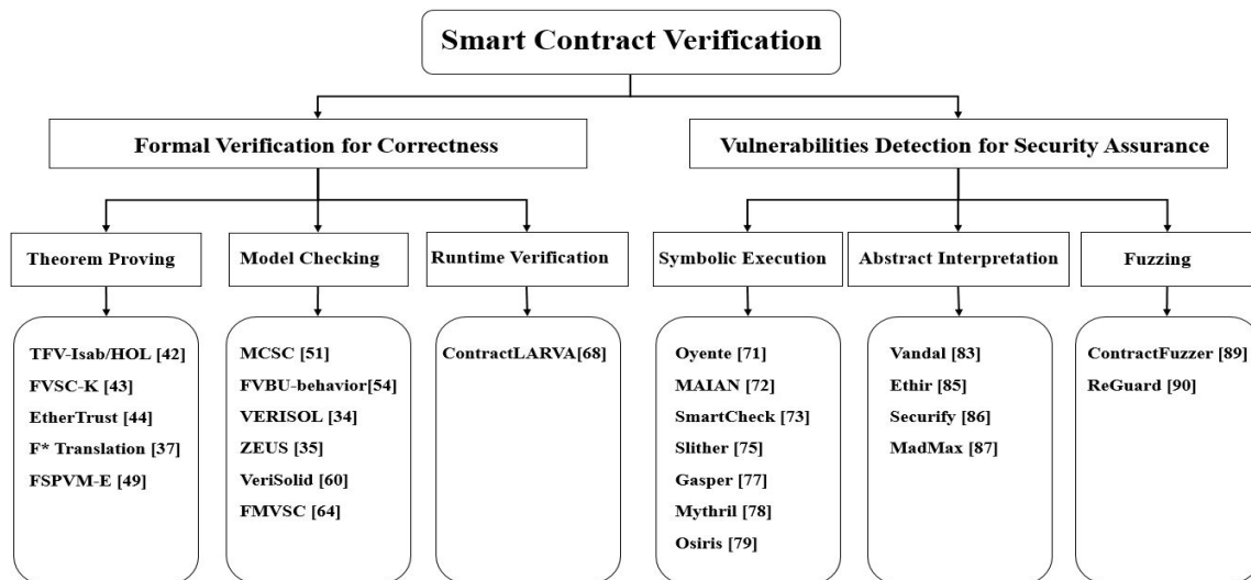
Figure 1: Taxonomy of the smart contract verification's Tools
