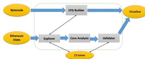
Figure 9: Oyente Workflow [71]
