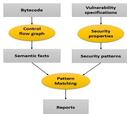
Figure 12: Securify Workflow
