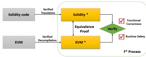
Figure 4: F* Architecture
