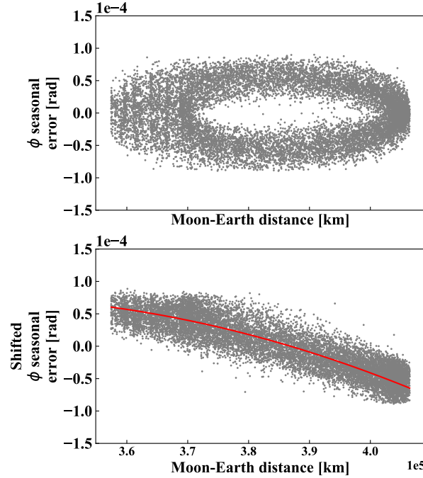
Figure 3: Along-track seasonal error as a function of Moon-Earth distance in 2018.
