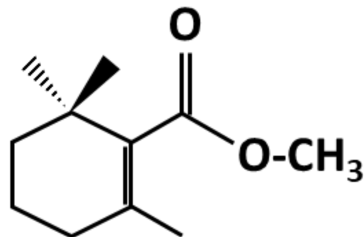
Methyl 2,6,6-trimethyl-1-cyclohexene-1-carboxylate
