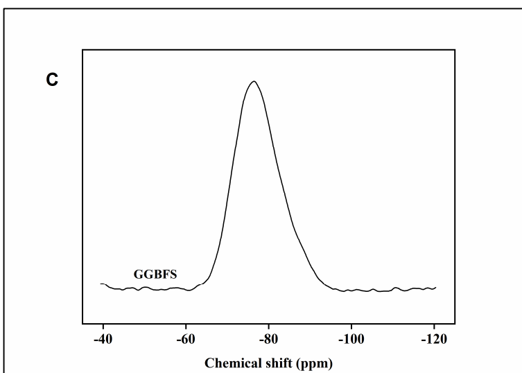
Figure A.3. ^{27}\text{Al} (A) and ^{29}\text{Si} MAS NMR of powders (B: Fly ash, C: GGBFS).
