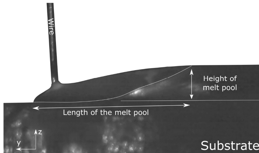
Fig. 3 - Picture from the high-speed camera illustrating the measurement of the length and height of the melt pool
