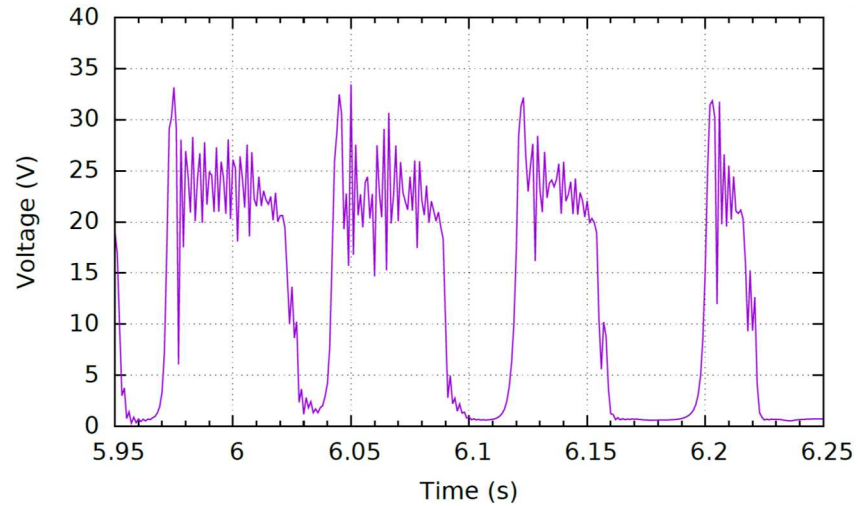
Fig. 10 -Evolution of the voltage during four metal transfer cycles.
