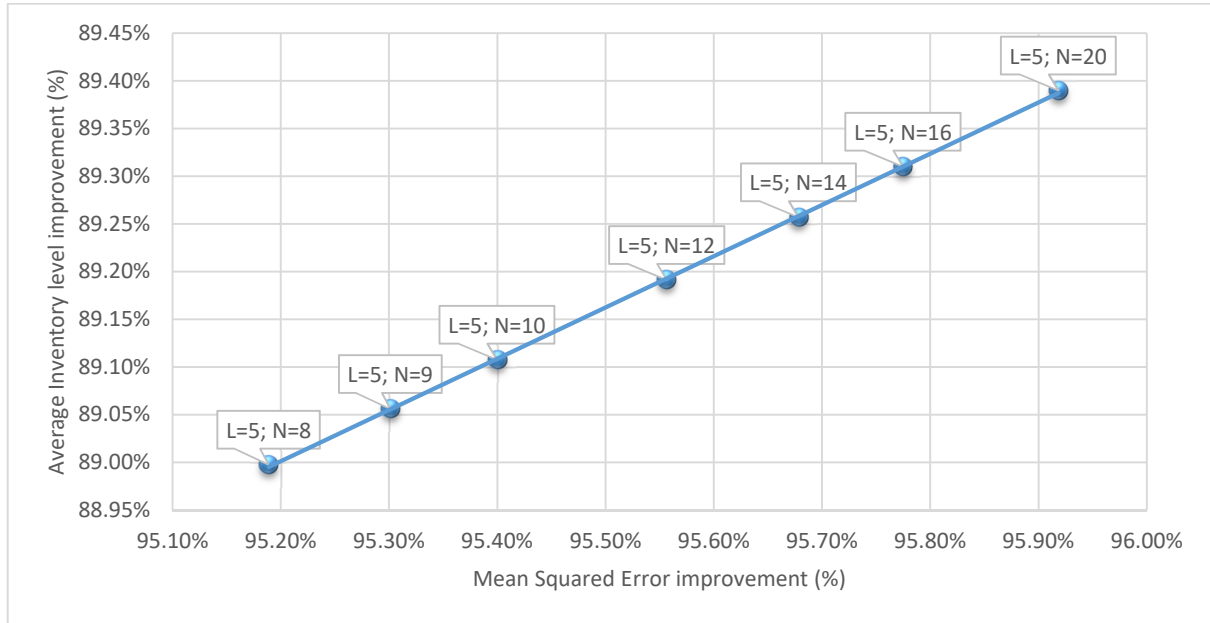
Figure 1: Improvements of adopting DDI strategy with WMA/Newton method rather than adopting NIS strategy according to the moving average parameter N
