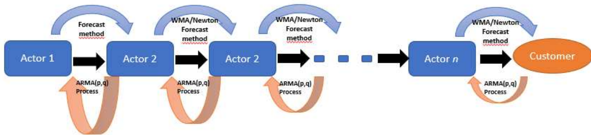
Figure 7: N-level supply chain where actors accept DDI while adopting WMA/Newton forecasting
