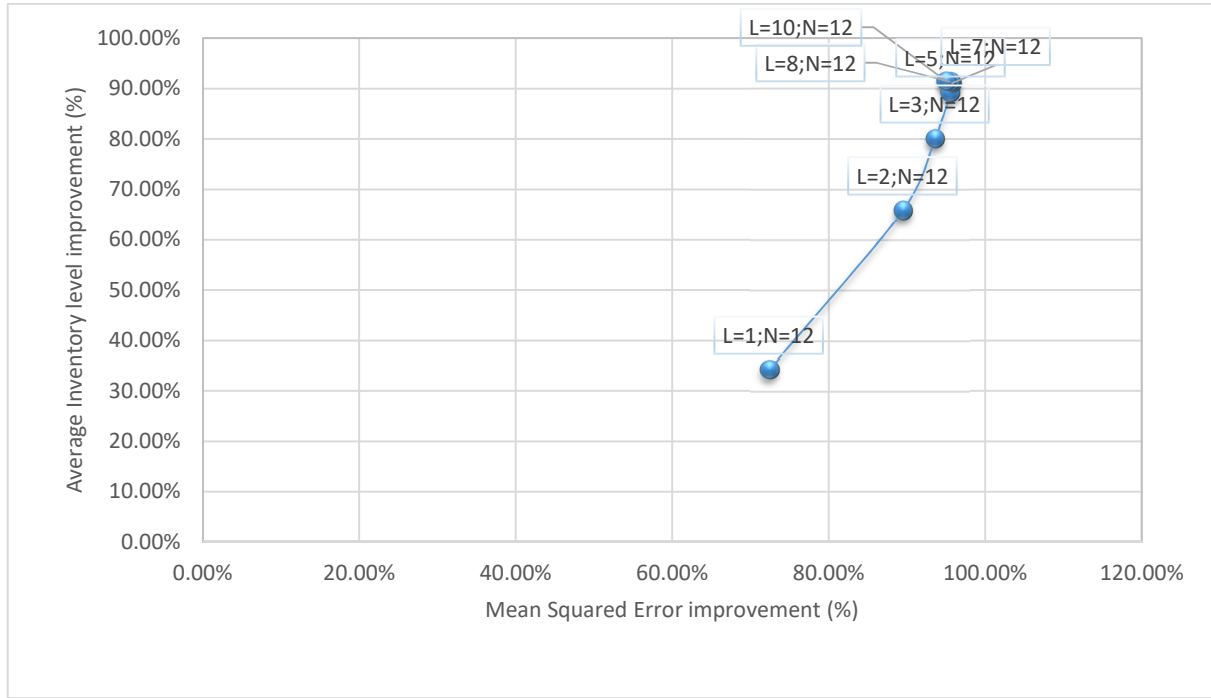
Figure 2: Improvements of adopting DDI strategy with WMA/Newton method rather than adopting NIS strategy according to the moving average parameter L
