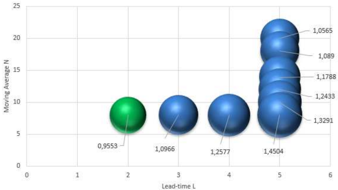
Figure 5: Simulated BEE_{MMSE}^{WMA/Newton} indicator according to moving average N and lead-time L
