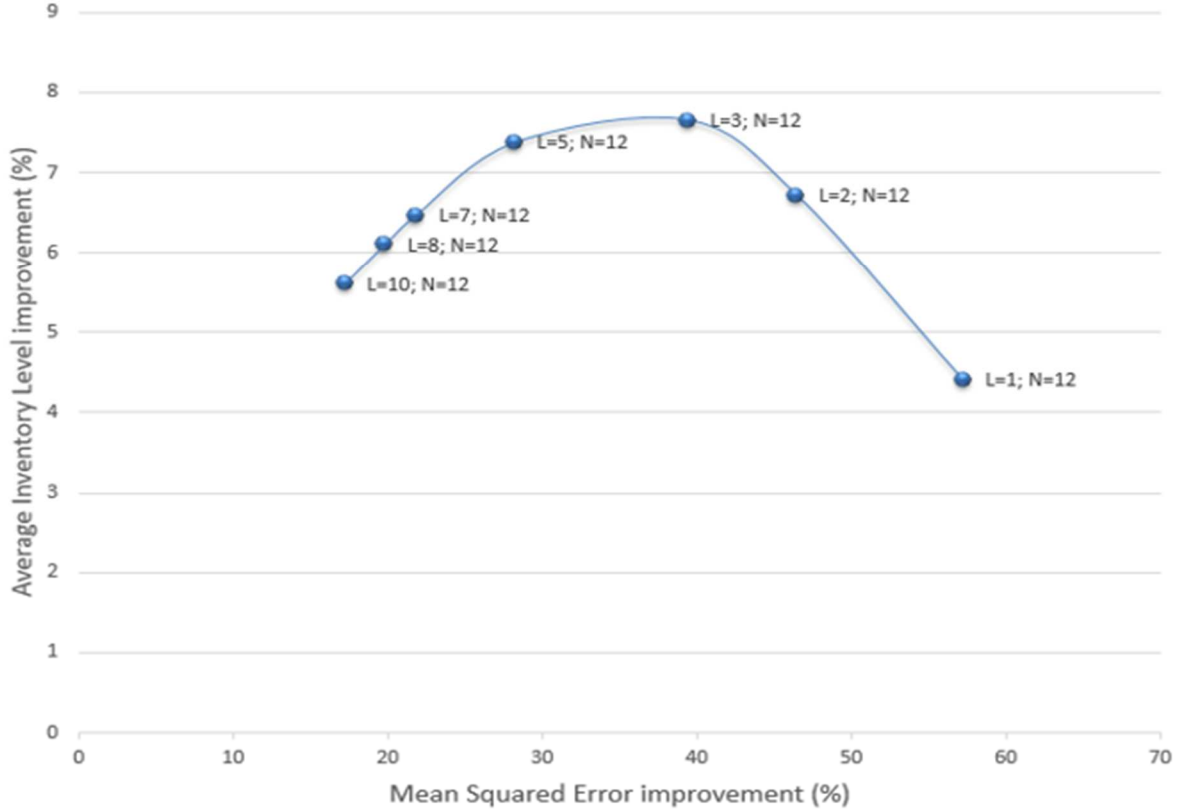
Figure 4: Improvements of adopting DDI strategy with WMA/Newton method rather than adopting DDI with SMA according to the lead-time L
