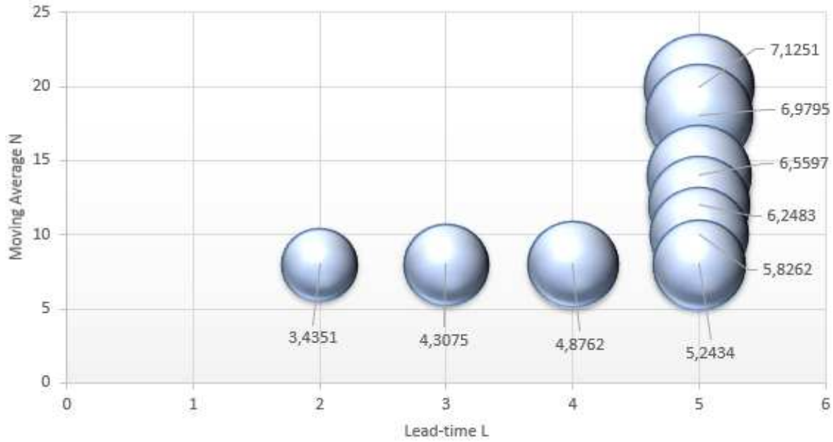
Figure 6: Simulated BEE_{SMA}^{WMA/Newton} indicator according to moving average N and lead-time L
