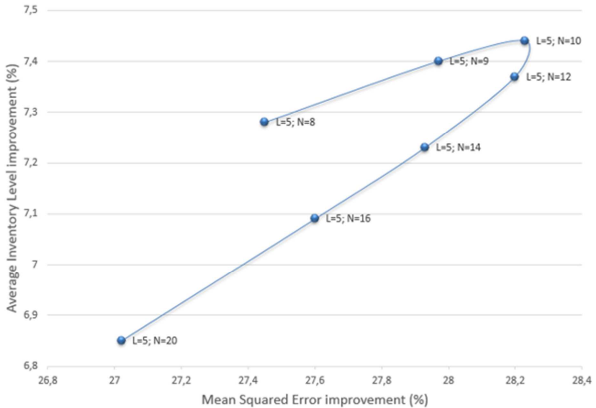
Figure 3: Improvements of adopting DDI strategy with WMA/Newton method rather than adopting DDI with SMA according to the moving average parameter N
