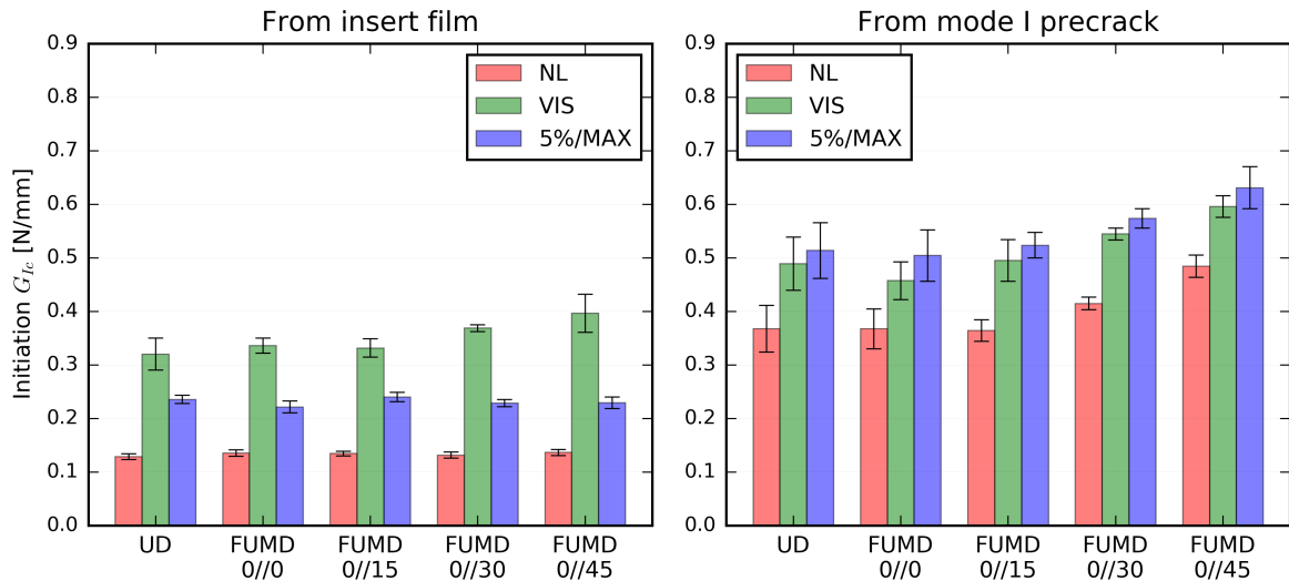
Figure 7: Initiation values of G_{Ic} .
