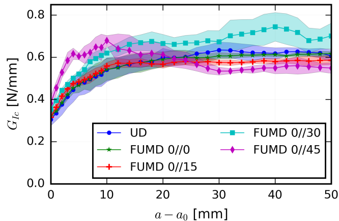
Figure 8: R-curves: average curve for all types of specimens and relative standard deviation.
