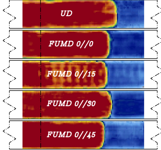
Figure 15: Representative C-scans for all sequences adopted. In this view, delamination propagated from the left to the right. The dashed line superposed to the C-scan images is the location of the insert tip.
