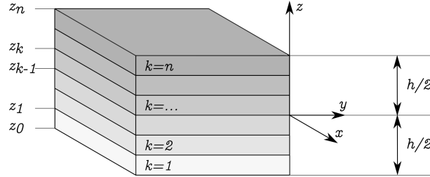
Figure 1: Laminate stacking parameters and notation.
