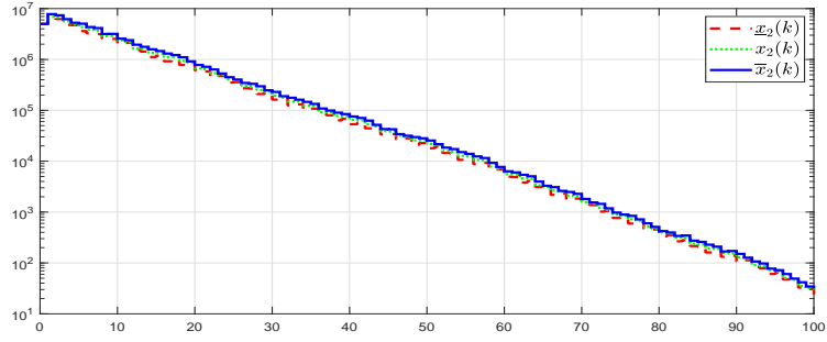
Figure 2: The simulations of the state x_2(k) and its upper and lower bounds
