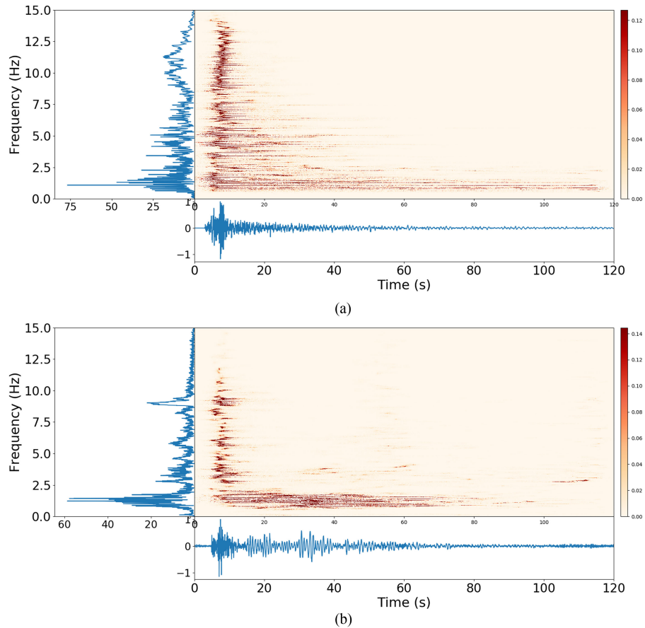
Fig. 8. Signals induced by the detonation of a 400-kg TNT-equivalent charge located on the seabed at 3TY (corresponding to the explosion S6), and recorded at the station PS13 located on the coast. They represent the horizontal component of the velocity (colinear to the source–receiver direction), together with their spectrograms. (a) Simulated data. (b) Real data. Note that as the real source function was not accounted for in the numerical simulations, the amplitude of the simulated data is only indicative and cannot be compared with the real data amplitude. The amplitudes of the time signals have been normalized.
