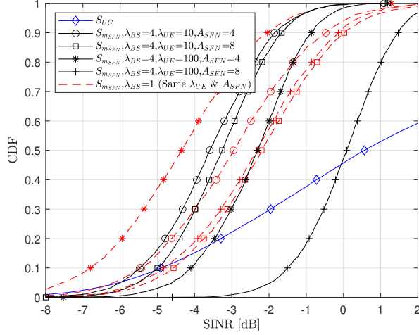
Figure 2: CDF of the minimum SINR to cover in MBSFN mode ( S_{mSFN} ) and CDF of the SINR in UC ( S_{UC} ) for different scenarios considering A_{MC} = 4 \text{ km}^2 . \lambda_{BS} in BS/km 2 , \lambda_{UE} in UE/km 2 and A_{SFN} in km 2 .
