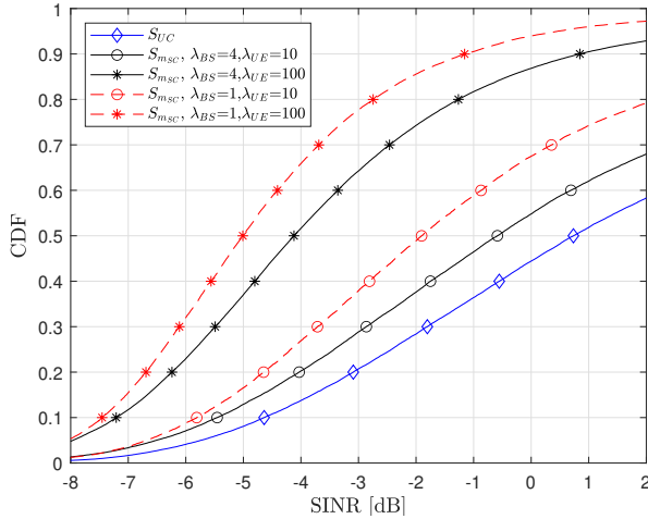
Figure 3: CDF of the minimum SINR to cover in SC-PTM mode ( S_{mSC} ) and CDF of the SINR in UC ( S_{UC} ) for different scenarios considering A_{MC} = 4 \text{ km}^2 . \lambda_{BS} in BS/km 2 and \lambda_{UE} in UE/km 2 .
