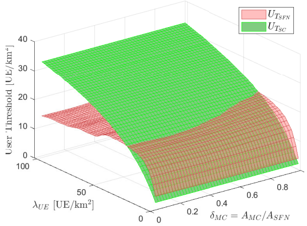
Figure 5: User threshold for MBSFN ( U_{T_{SFN}} ) and SC-PTM ( U_{T_{SC}} ) for different scenarios considering \lambda_{BS} = 4 \text{ BS/km}^2 and A_{MC} = 4 \text{ km}^2 .
