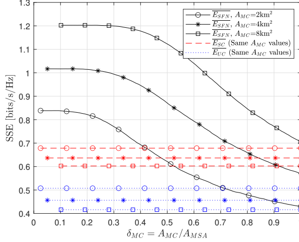
Figure 4: System Spectral Efficiency in MBSFN, SC-PTM and Unicast transmission modes for different scenarios considering \lambda_{BS} = 4 \text{ BS/km}^2 and \lambda_{UE} = 100 \text{ UE/km}^2 .
