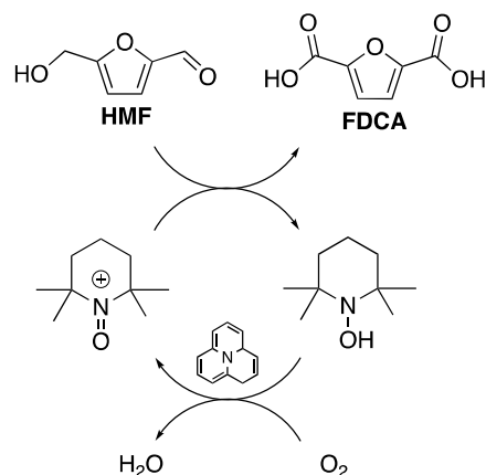
Scheme 6. Possible reaction pathway for oxidation of HMF in NG-TEMPO catalytic system.
