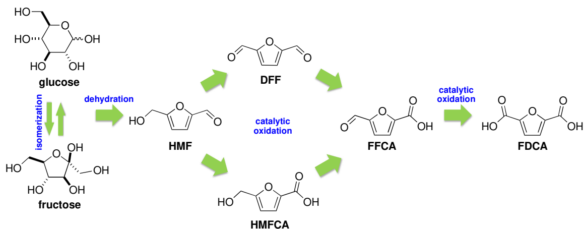
Scheme 1. Oxidation pathway for HMF.
