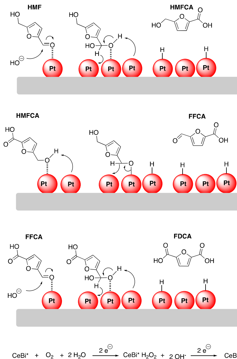
Scheme 5. The proposed reaction mechanism for the oxidation of HMF with CeBi* representing the oxygen vacancy accompanied with the bismuth.
