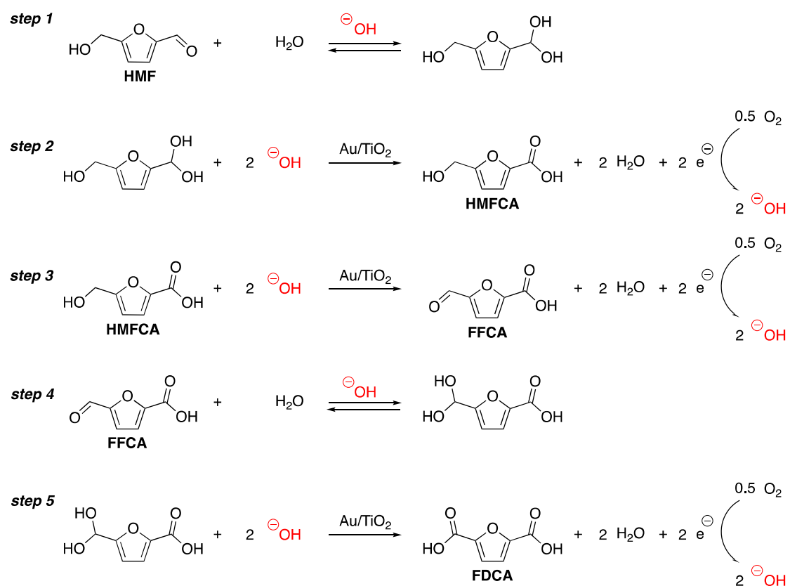
Scheme 3. Overall mechanism for oxidation of HMF-to FDCA.
