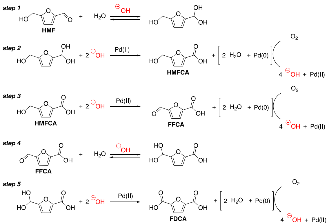
Scheme 4. Aerobic oxidation of HMF into FDCA over Pd catalyst.
