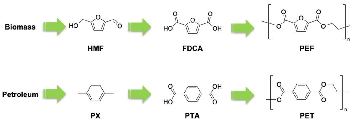
Scheme 2. The comparative origins of PEF and PET.
