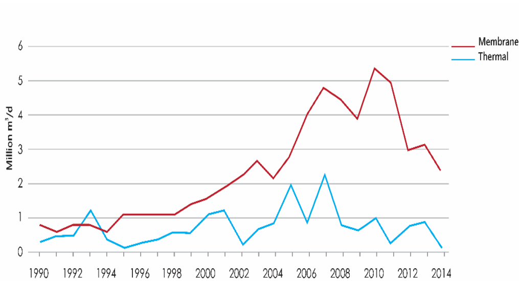
Fig 11: Awarded membrane and thermal desalination capacity, 1990–2014 [73].
