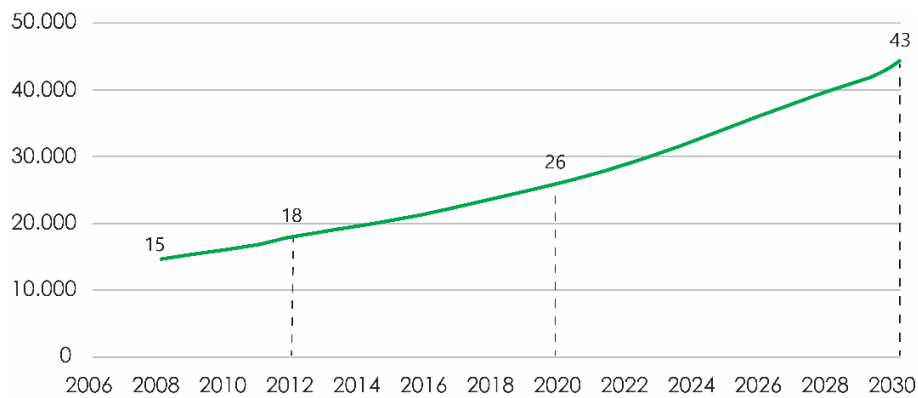
Fig 2: Morocco's primary energy demand in Millions TEP [25].
