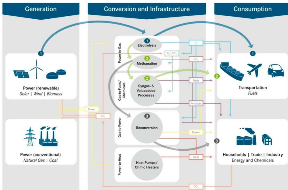
Fig 9: Power-to-X applications [67]
