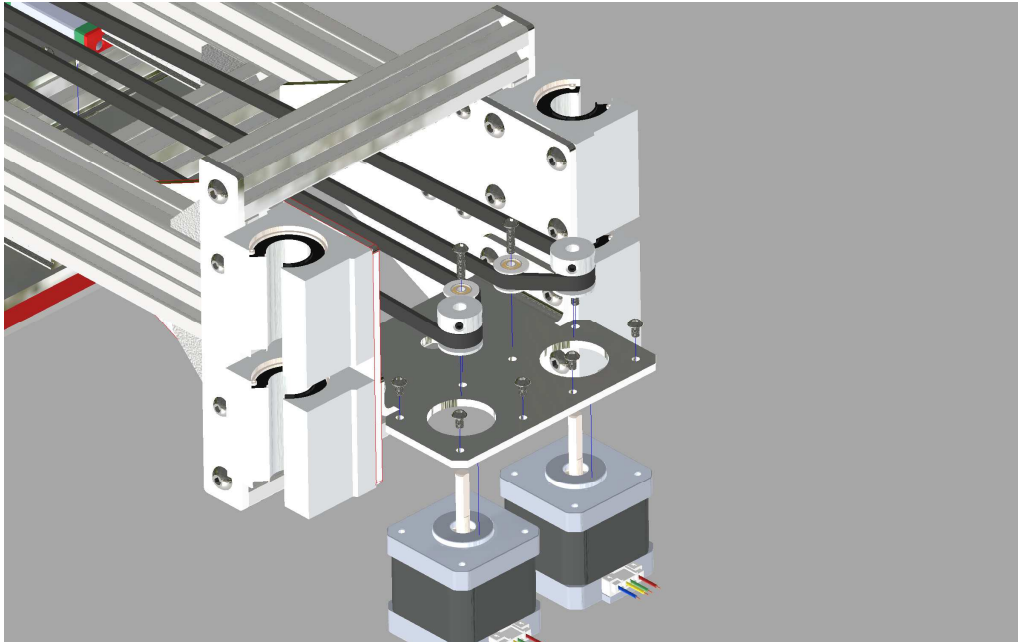
Figure 7. Motor and pulley mounts
