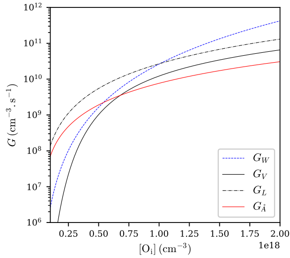
Fig. 3: TD formation rates as a function of [O_i] (using a FTIR calibration coefficient of 3.14 \times 10^{17} \text{ cm}^{-2} ). The temperature was set to 420 \text{ }^\circ\text{C} (i.e. the highest temperature investigated in [20]).
