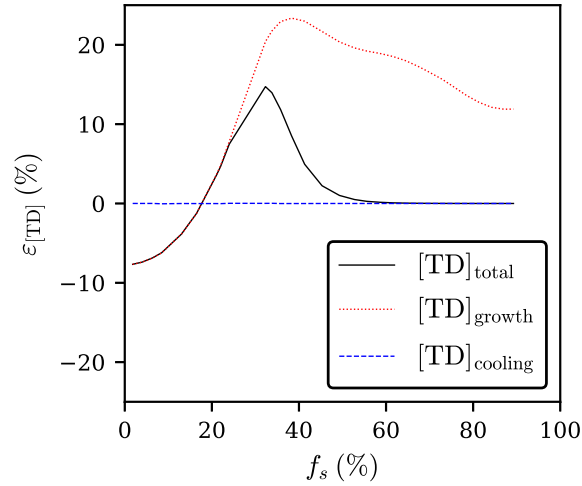
Fig. 10: Relative deviation between TD concentrations computed with a constant pulling rate and TD concentrations computed with the experimental pulling rate values, \epsilon_{[TD]} = \{[TD]_{constant\ rate} - [TD]_{variable\ rate}\} / [TD]_{variable\ rate} , for the ingot 1.
