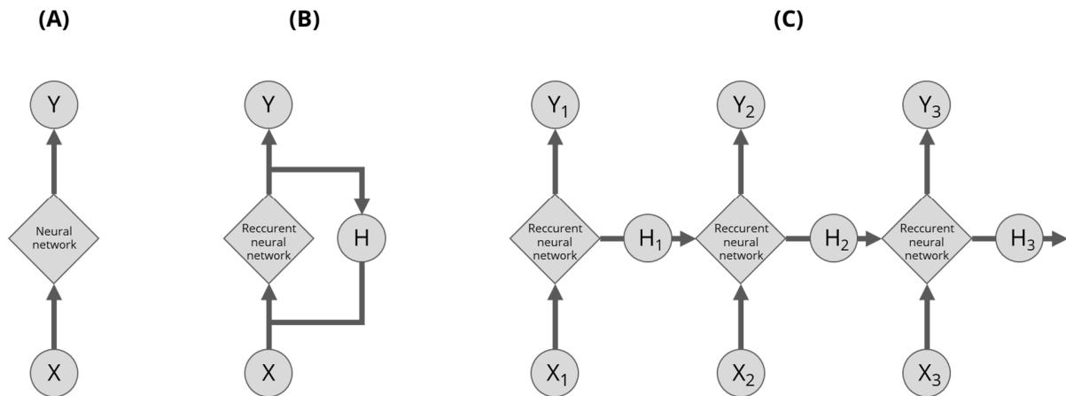
Figure 2 – Classic feedforward neural network (A), recurrent neural network (B), and “unrolled” graphical representation of a recurrent neural network (C) where we use sequence data (x_1, x_2, x_3) to make sequence predictions (y_1, y_2, y_3) while preserving information through the hidden states h_1, h_2, h_3 .
