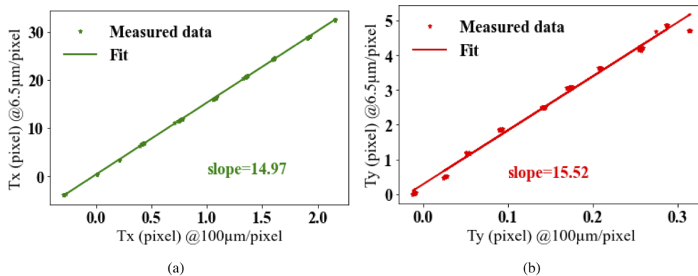
Fig. 7. Measured x (a) and y (b) translations at high resolution as functions of measured translations at low resolution. The measured slopes are about 15 as expected from the resolution change.
