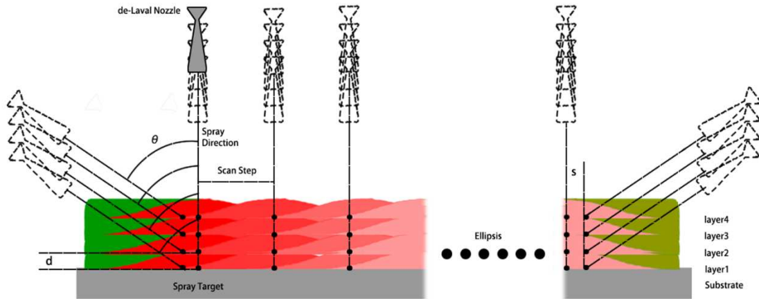
Fig. 11. Schematic of CSAM spray strategy for large blocks or thick coatings
