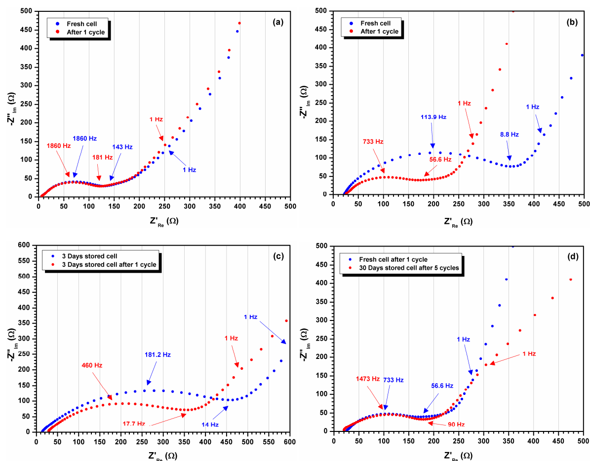
Fig. 10. (a) EIS profiles at 3.2 V of LMO//Li half-cells filled with LiPF 6 1.5 M in EC/EMC (3/7). (b,c,d) EIS profiles at 3.2 V of freshly prepared or stored (25 °C) of LMO//Li half-cells filled with 1.5 M LiPF 6 in EC/EMC/TFEMC (3/4/3).
