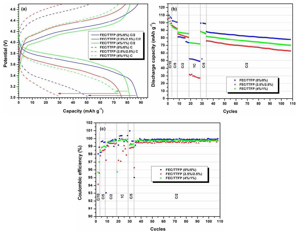
Fig. 4. (a) Galvanostatic profiles at C/2 and C of Gr//LMO cells cycled between 3.0 and 4.7 V at room temperature with 1.5 M \text{LiPF}_6 in EC/EMC (3/7, w/w), and two combination of FEC-TTFP as additive. (b) Corresponding discharge capacities. (c) Corresponding coulombic efficiencies.
