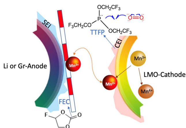
Scheme 1. Schematic presentation for the protective action of delithiated LMO cathode by TTFP and Li or Gr anode by FEC toward manganese dissolution and attack.
