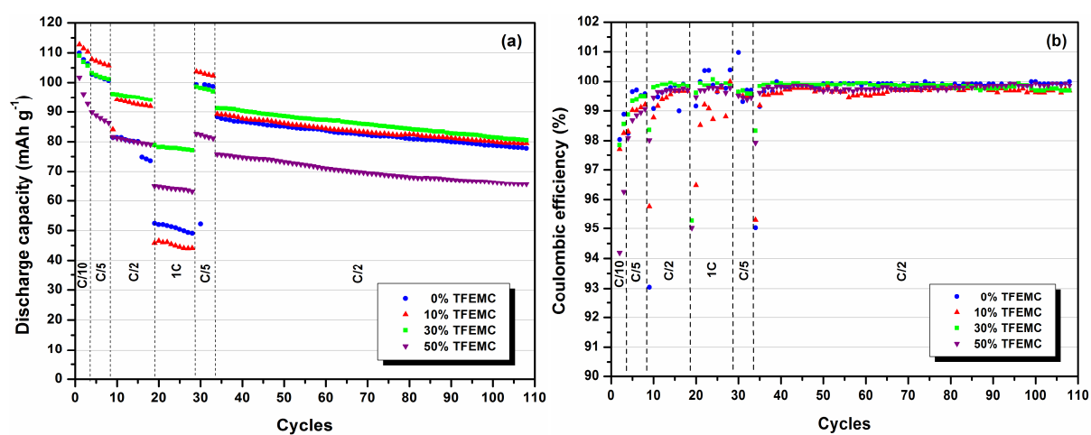
Fig. 9. (a) Discharge capacities of Gr//LMO cells cycled between 3.0 and 4.7 V at room temperature with LiPF 6 1.5 M in EC/EMC/TFEMC (3/7- x/x ) with x = 0,1,3,5. (b) Corresponding coulombic efficiencies.
