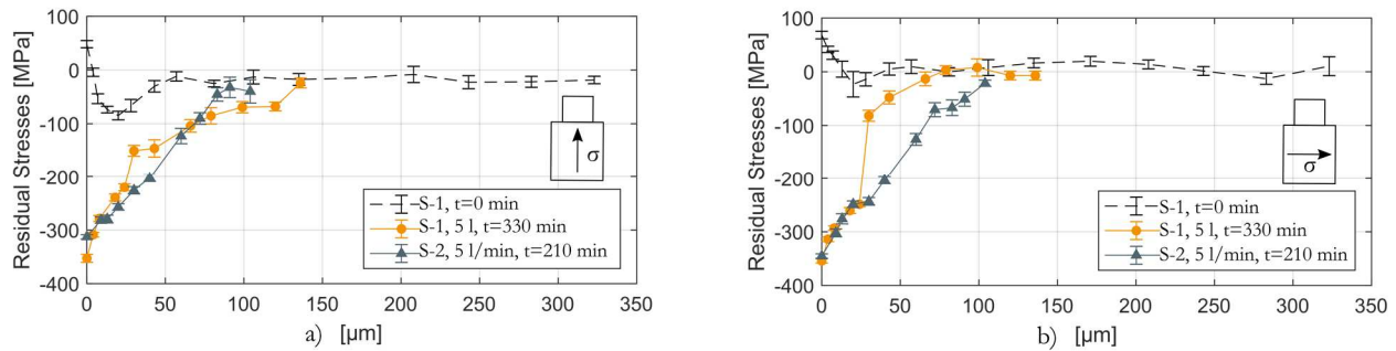
Fig. 7. Residual stress profiles in S-1 and S-2, in a) axial direction and b) circumferential direction.
