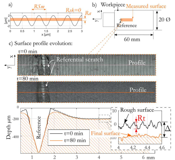
Fig.3. a) A periodical rough surface indicating R_a , RSm and Rsk , b) sample geometry, and c) measurement strategy for surface profile superposition, a case where the initial topography has been totally removed.
