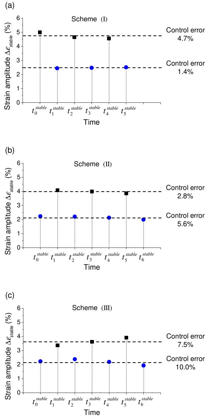
Figure 7. The strain amplitude scattering in Schemes I, II and III. The control error is defined
