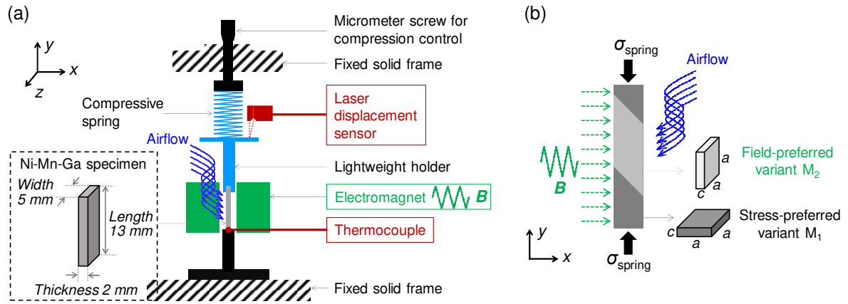
Figure 1. Schematics of (a) the experimental setup of the thermo-magneto-mechanical coupling actuation system and (b) the martensite reorientation of MSMA.
