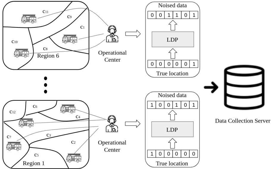
Figure 3: An outline of the approach applied to collect firemen intervention's location data preserving privacy.
