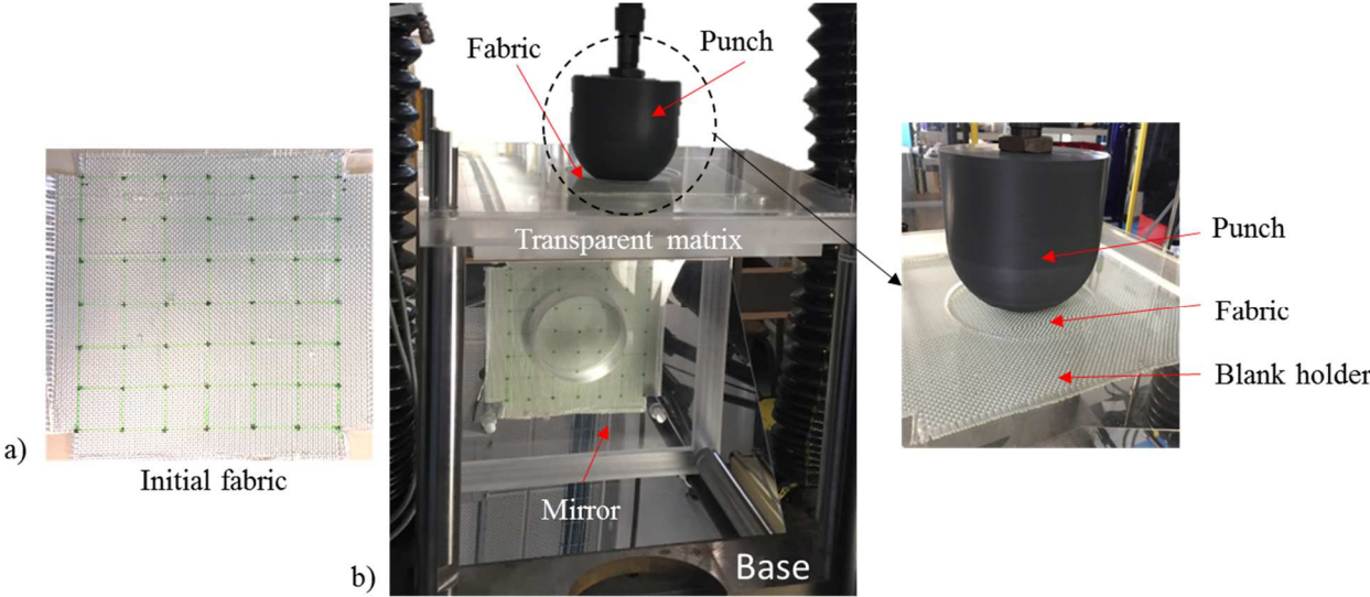
Fig.10 a) Initial fabric and b) Experimental device for hemispherical stamping
