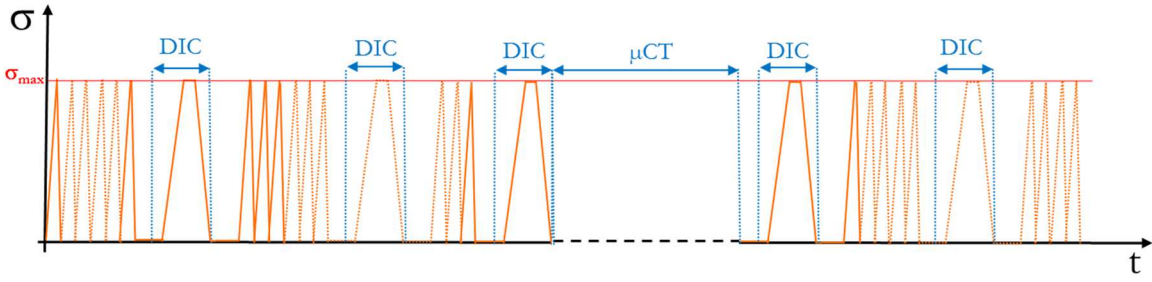
Figure 2: Schematic fatigue test cycle. Fatigue tests are periodically interrupted to perform DIC measures and \mu CT scans.
