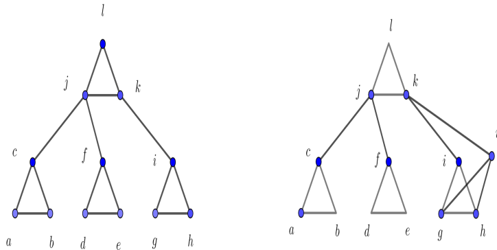
FIGURE 4. \text{dstab}(I_G) = 5
