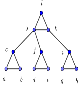
FIGURE 2. (a^2, \dots, l^2) is not an irreducible component of I_G^6
