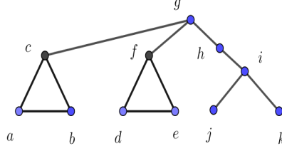
FIGURE 1. I_G has 22 irreducible components
