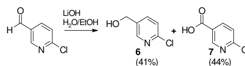
Scheme 3. Cannizzaro reaction of 6-chloro-pyridine-3-carbaldehyde.
