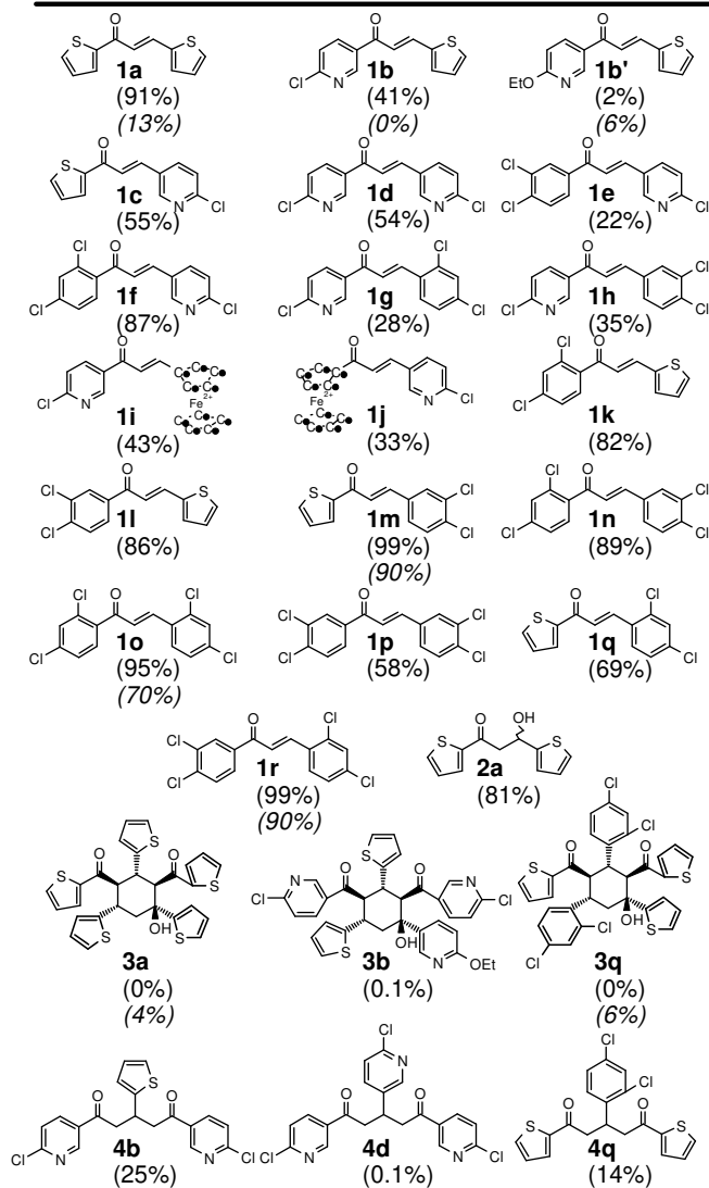
Scheme 1. Claisen-Schmidt condensation of (hetero-)aryl ketones and (hetero-)aryl aldehydes, and compounds synthesized in this study (yields are given within brackets, relatively to aldehyde and ketone reagents; regular writing correspond to ultrasounds mediated experiments, and italic writing correspond to classical stirring experiments).
