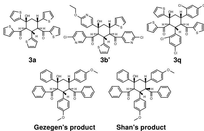
Figure 3. Structure of cyclohexanols 3a , 3b' and 3q compared to literature equivalents.
