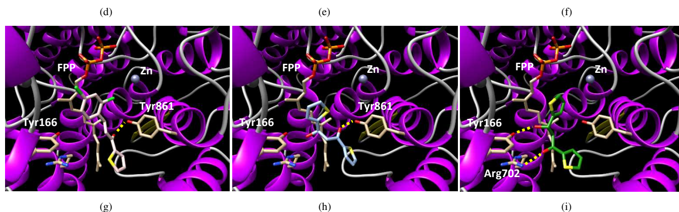
Figure 4. Docking of synthesized molecules in the active site of human farnesyltransferase: chalcone 1i (a), chalcone 1j (b), chalcone 1k (c), chalcone 1l (d), chalcone 1p (e-f), chalcone 1q (g) and \beta -hydroxy-ketone 2a (enantiomer R (h); enantiomer S (i)). Yellow dashed lines represent hydrogen bonds between investigated molecules and aminoacids present in the active site of human farnesyltransferase.
