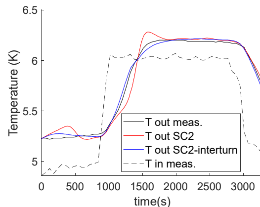
Fig. 12 –Comparison between measured TF inlet & outlet temperature profiles (black curves) and Simcryogenics results using SC2 model with inter-turn thermal coupling (blue curve) and without inter-turn thermal coupling (red curve).
