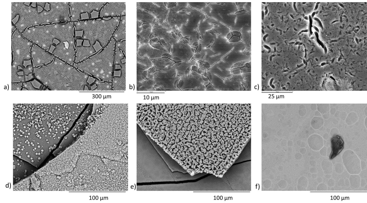
Figure 7. SEM-BSE images of the previous surfaces of a) 20pH3, b) 20pH6.7, c) 20pH10, d) 70pH3, e) 70pH6.5 and f) 70pH8.5.
