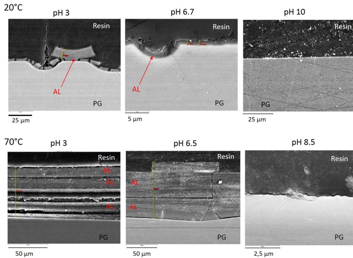
Figure 8. SEM-SE cross-sections images of samples altered at 20 and 70°C during 74 days (67 days for 70pH6.5). "AL" means Altered Layer and "PG" means Pristine Glass.
