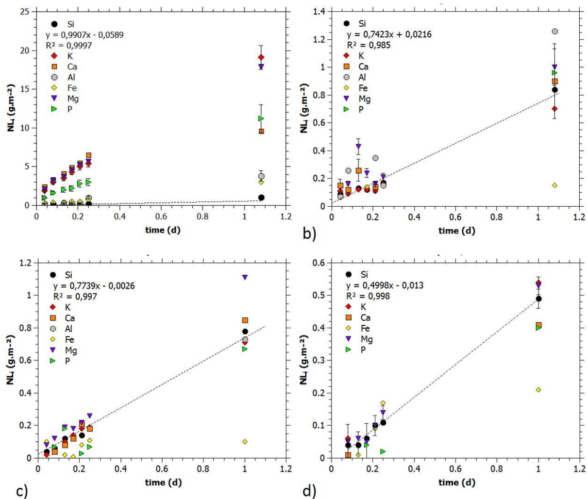
Figure 1. Normalized mass losses of glass elements i ( NL_i in g \cdot m^{-2} ) for samples altered at 50°C at pH: a) 2.0 b) 5.4 c) 6.3 and d) 9.8 for 24 h in static condition. Black regression lines correspond to Si evolution. Uncertainties are low and corresponding error bars are sometimes smaller than symbols.
