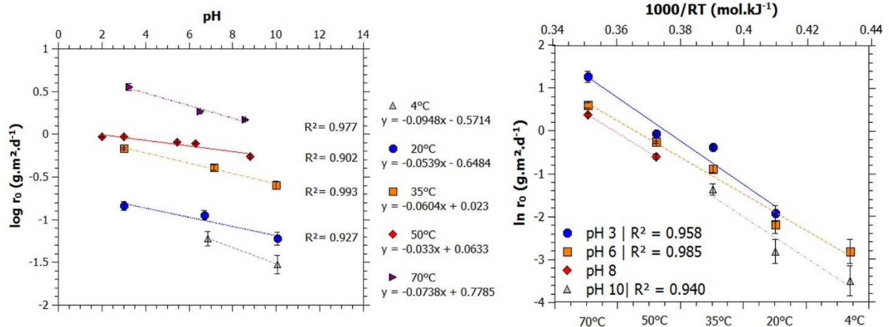
Figure 3. a ) Logarithm of initial dissolution rate r_0 (in \text{g.m}^{-2}.\text{d}^{-1} ) as a function of pH for the experiments at 20, 35, 50 and 70°C. b ) Natural logarithm of initial dissolution rate r_0 (in \text{g.m}^{-2}.\text{d}^{-1} ) as a function of 1000/RT (in \text{mol.kJ}^{-1} ) for pH 3, 6, 8 and 10. Values of n , k_0 and E_a are indicated in Tables 5 and 5.
