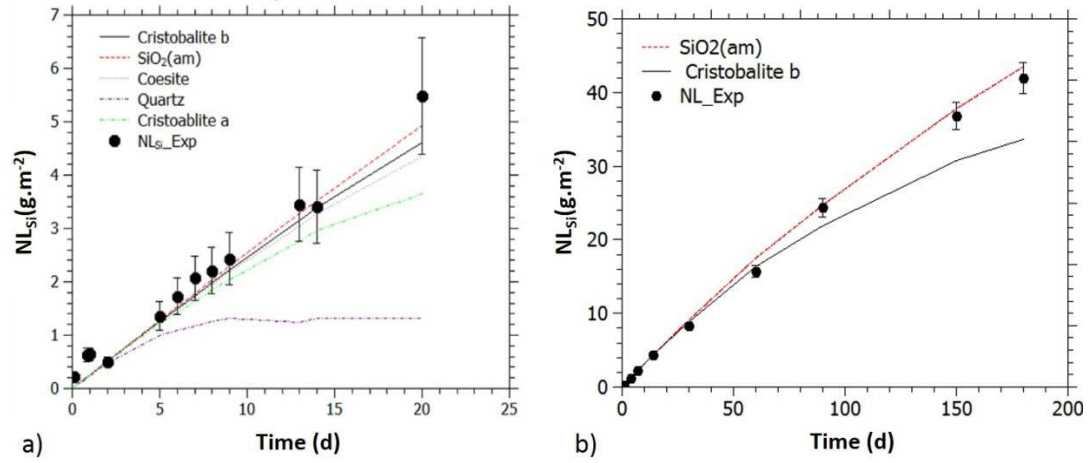
Figure 5. Fits of experimental NL_{Si} (black points) with dissolution rate law (Eq. 4) including ro\_measured (Table 4) and several silica phases tested for the chemical affinity term. a) Sample altered at pH 10 and 35°C during 20 days. b) Fit of experimental NL_{Si} from Sessegolo et al., 2019.
