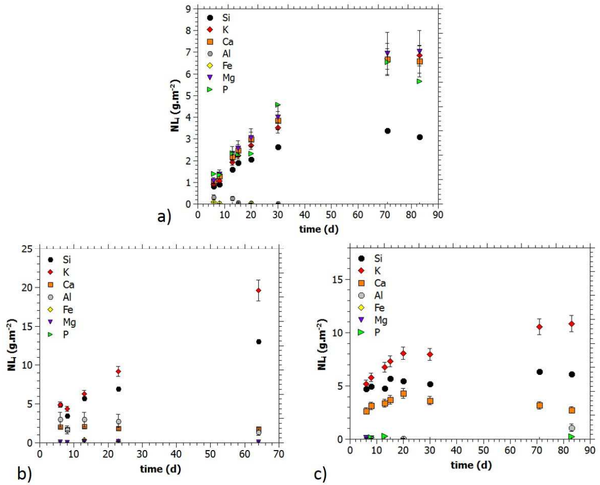
Figure 2. Normalized mass losses of glass elements i ( NL_i in \text{g.m}^{-2} ) for samples altered at a) 20°C and pH 10.3, b) 70°C at pH 9.8 and c) 70°C at pH 10.4 in static condition. Uncertainties can be low and corresponding error bars are sometimes smaller than symbols. For c) numerous elemental concentrations were lower than the quantification limits.
