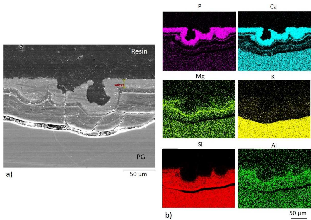
Figure 9. 70pH6.5 SEM-EDS analysis after 67 days of alteration. a) SEM-BSE image of the alteration layer, b) EDS mapping.
