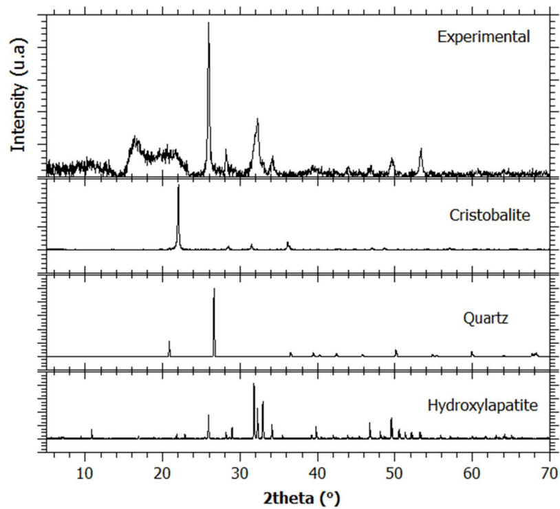
Figure 10. Diffractogram of experimental phases present on the surface of the sample altered at 70°C and pH 3 for 67. The reference one of quartz, cristobalite \alpha and hydroxylapatite (XRD) are presented.
