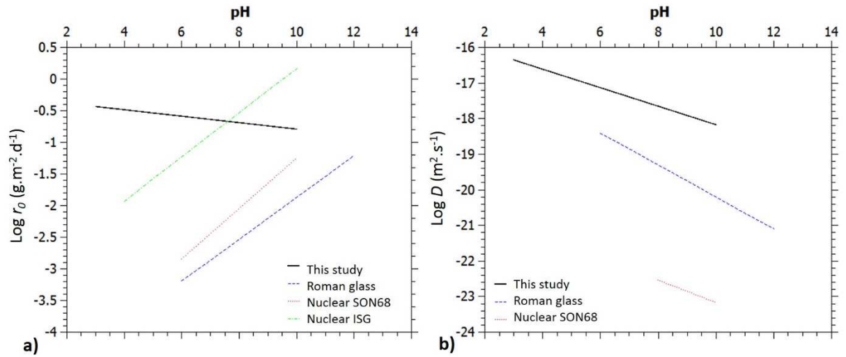
Figure 11. Theoretical evolution of dissolution and interdiffusion rate as a function of pH for different glass compositions. a) Logarithm of the initial dissolution rate r_0 according to the rate laws of this study (medieval-model type glass), Advocat et al., 1990 (SON68 nuclear glass), Inagaki et al., 2013 (ISG nuclear glass) and Verney-Carron et al., 2010 (Roman glass). Calculations were carried out at 25°C. b) Logarithm of the diffusion of K (this study), Na (Verney-Carron et al., 2010) (Roman glass) and B (Chave et al., 2007) (SON68 nuclear glass). Calculations were carried out at 30°C.
