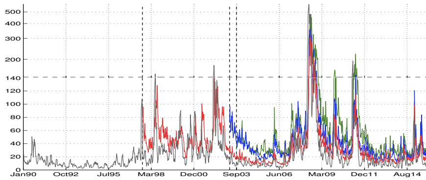
(b) VIX_{t,t+\tau}^2, VXD_{t,t+\tau}^2, VXX_{t,t+\tau}^2, RVX_{t,t+\tau}^2
