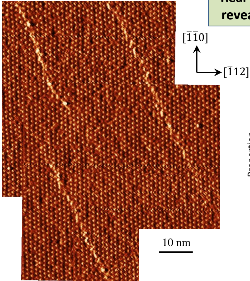
STM image of Nb single crystal surface strained at 90 K
